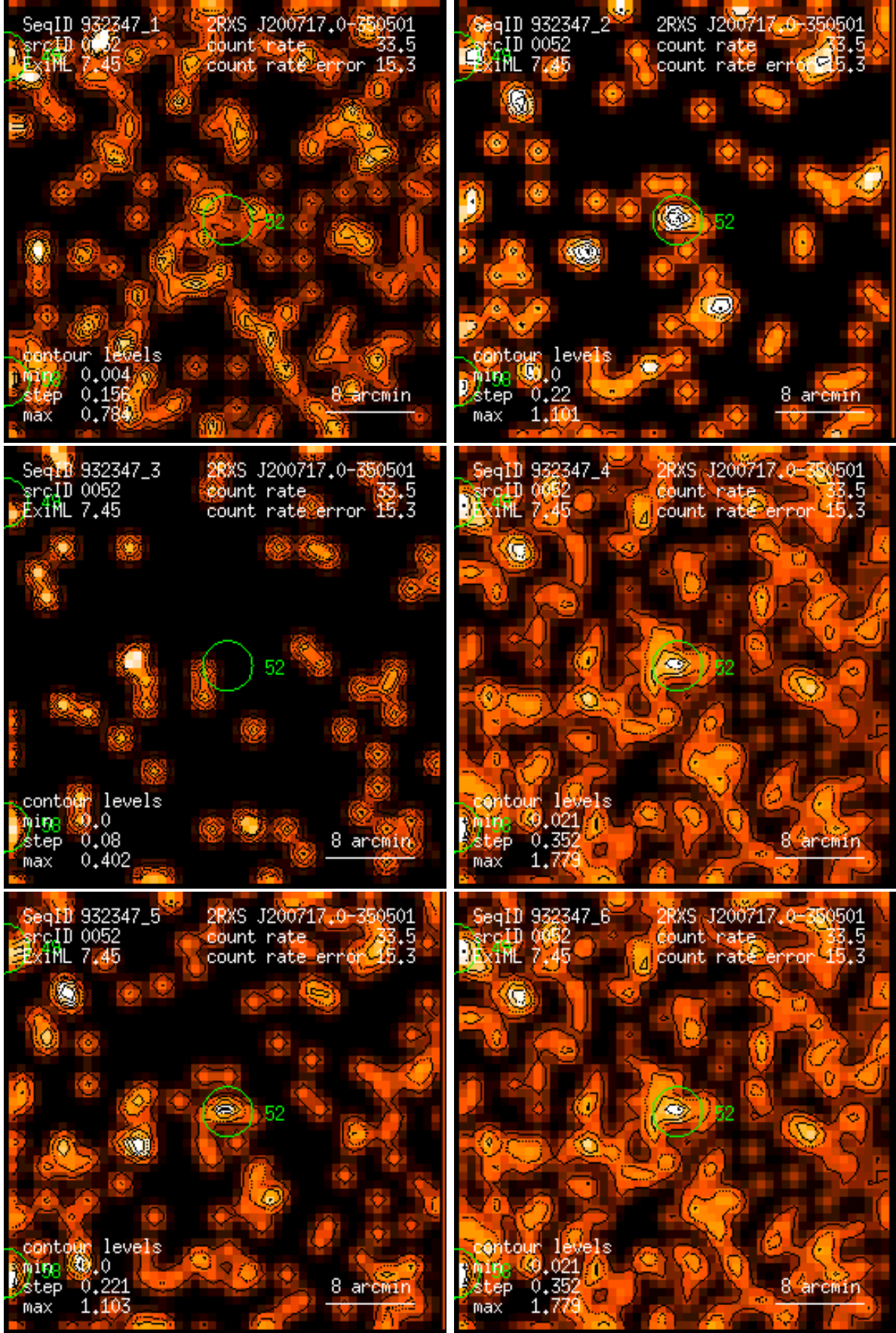
Figure 52: RASS 932347: detection 0052: band rate images, Gaussian filter: (1) PSPC channels 11 – 41, (2) 52 – 90, (3) 91 – 201, (4) 11 – 235, (5) 52 – 201, (6) 11 – 201. Broad band rates in counts/ks. Band rate contour levels in counts/ks/arcmin 2 .
