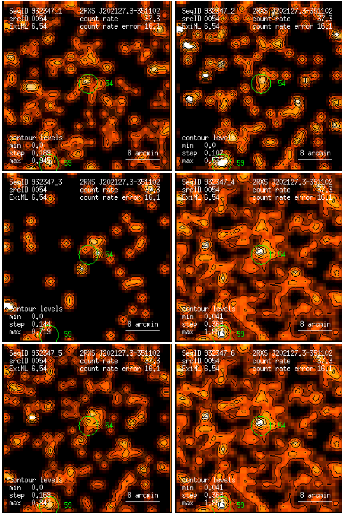
Figure 54: RASS 932347: detection 0054: band rate images, Gaussian filter: (1) PSPC channels 11 – 41, (2) 52 – 90, (3) 91 – 201, (4) 11 – 235, (5) 52 – 201, (6) 11 – 201. Broad band rates in counts/ks. Band rate contour levels in counts/ks/arcmin 2 .
