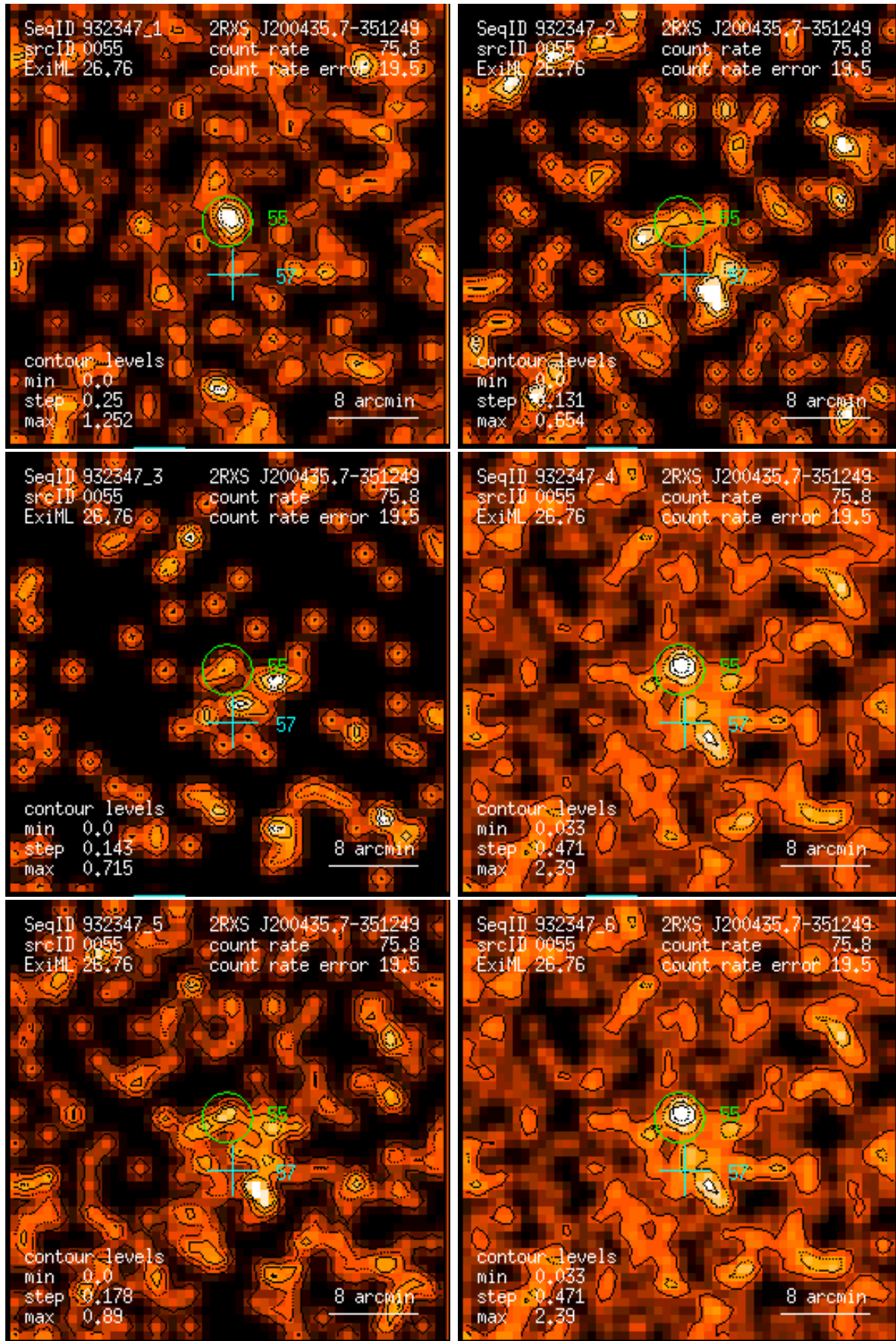
Figure 55: RASS 932347: detection 0055: band rate images, Gaussian filter: (1) PSPC channels 11 – 41, (2) 52 – 90, (3) 91 – 201, (4) 11 – 235, (5) 52 – 201, (6) 11 – 201. Broad band rates in counts/ks. Band rate contour levels in counts/ks/arcmin 2 .
