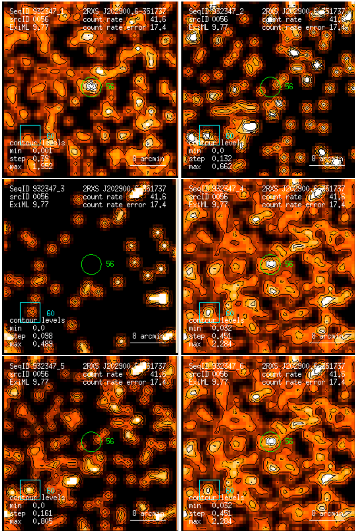
Figure 56: RASS 932347: detection 0056: band rate images, Gaussian filter: (1) PSPC channels 11 – 41, (2) 52 – 90, (3) 91 – 201, (4) 11 – 235, (5) 52 – 201, (6) 11 – 201. Broad band rates in counts/ks. Band rate contour levels in counts/ks/arcmin 2 .
