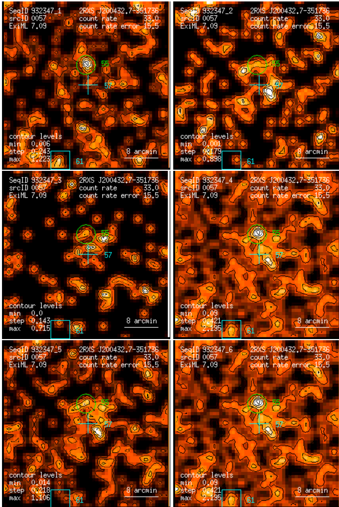
Figure 57: RASS 932347: detection 0057: band rate images, Gaussian filter: (1) PSPC channels 11 – 41, (2) 52 – 90, (3) 91 – 201, (4) 11 – 235, (5) 52 – 201, (6) 11 – 201. Broad band rates in counts/ks. Band rate contour levels in counts/ks/arcmin 2 .
