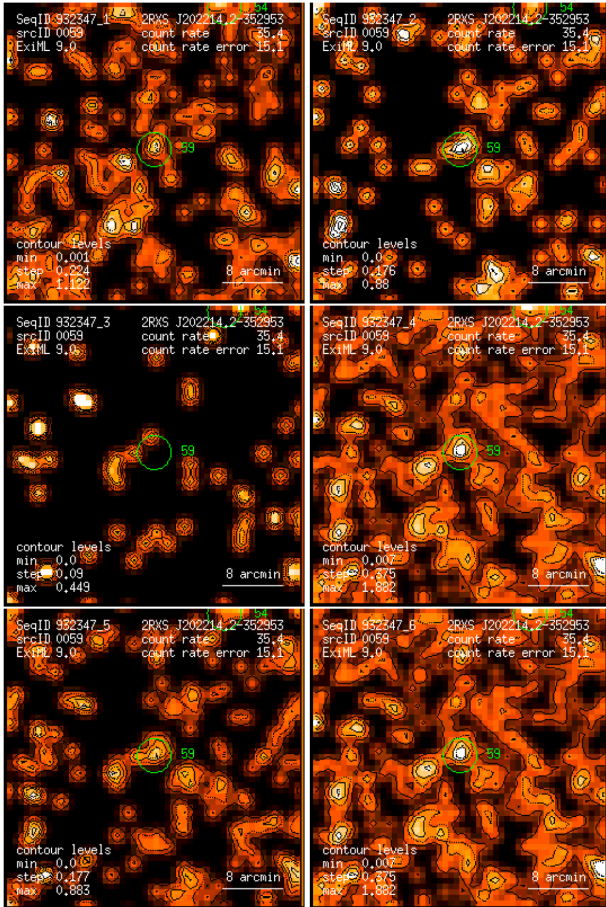
Figure 59: RASS 932347: detection 0059: band rate images, Gaussian filter: (1) PSPC channels 11 – 41, (2) 52 – 90, (3) 91 – 201, (4) 11 – 235, (5) 52 – 201, (6) 11 – 201. Broad band rates in counts/ks. Band rate contour levels in counts/ks/arcmin 2 .
