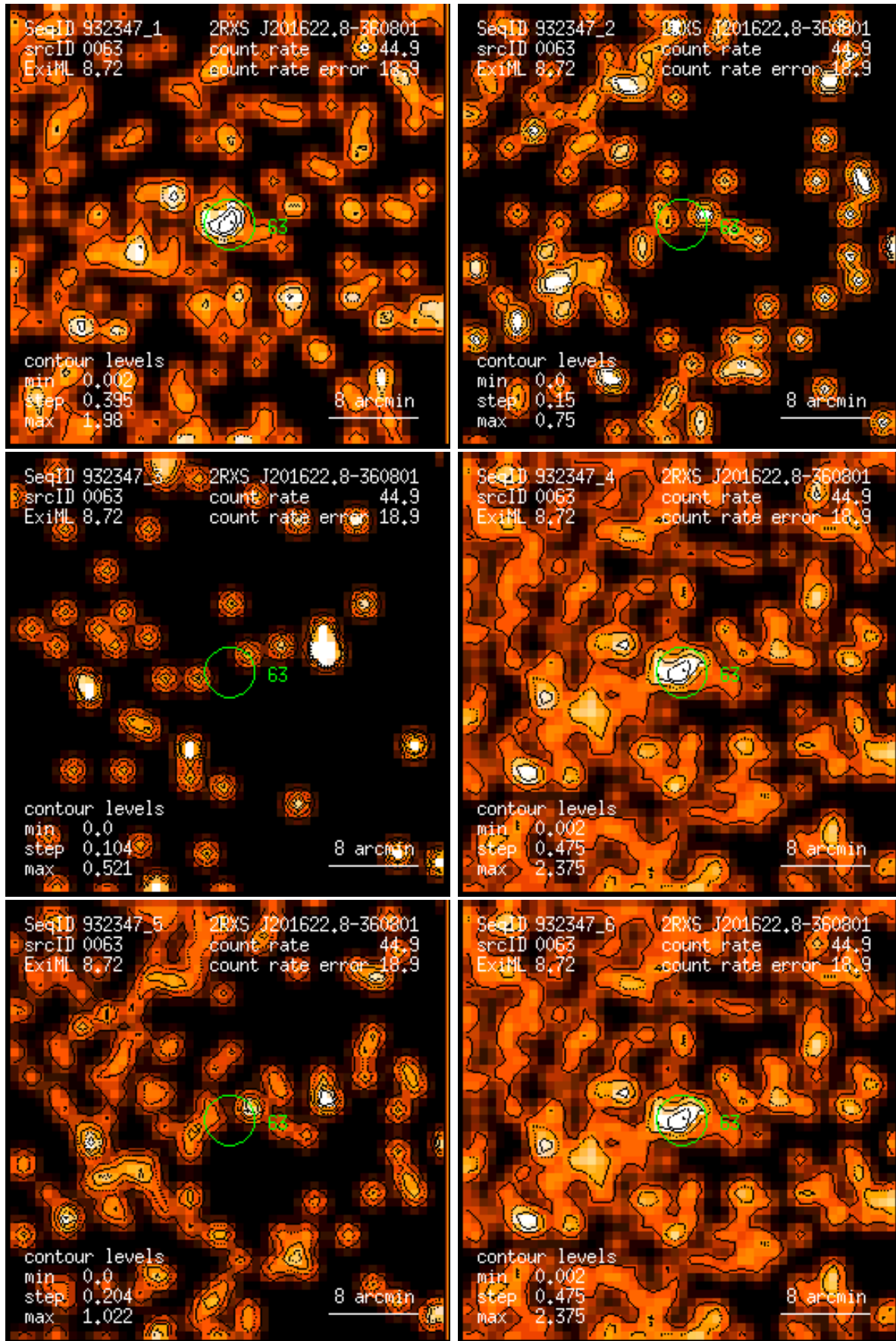
Figure 63: RASS 932347: detection 0063: band rate images, Gaussian filter: (1) PSPC channels 11 – 41, (2) 52 – 90, (3) 91 – 201, (4) 11 – 235, (5) 52 – 201, (6) 11 – 201. Broad band rates in counts/ks. Band rate contour levels in counts/ks/arcmin 2 .
