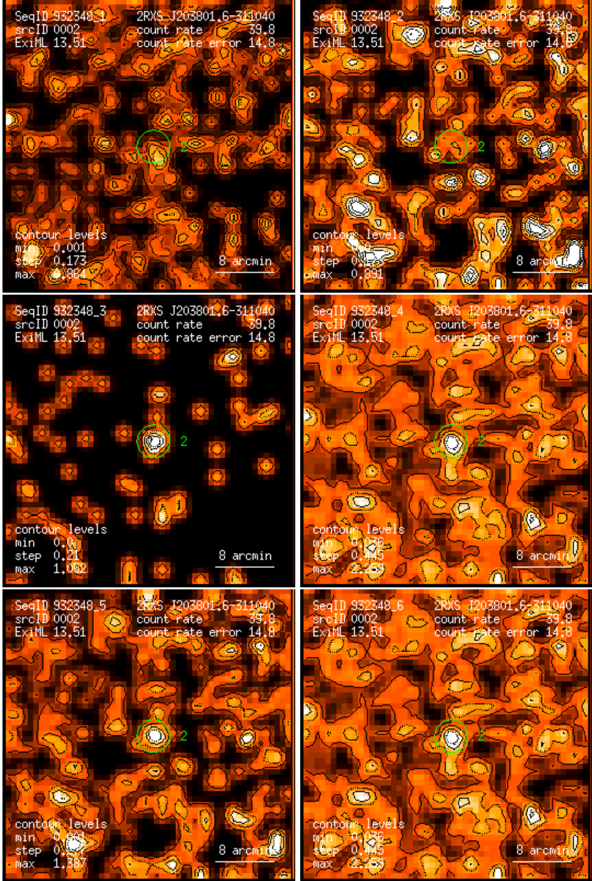
Figure 2: RASS 932348: detection 0002: band rate images, Gaussian filter: (1) PSPC channels 11 – 41, (2) 52 – 90, (3) 91 – 201, (4) 11 – 235, (5) 52 – 201, (6) 11 – 201. Broad band rates in counts/ks. Band rate contour levels in counts/ks/arcmin 2 .
