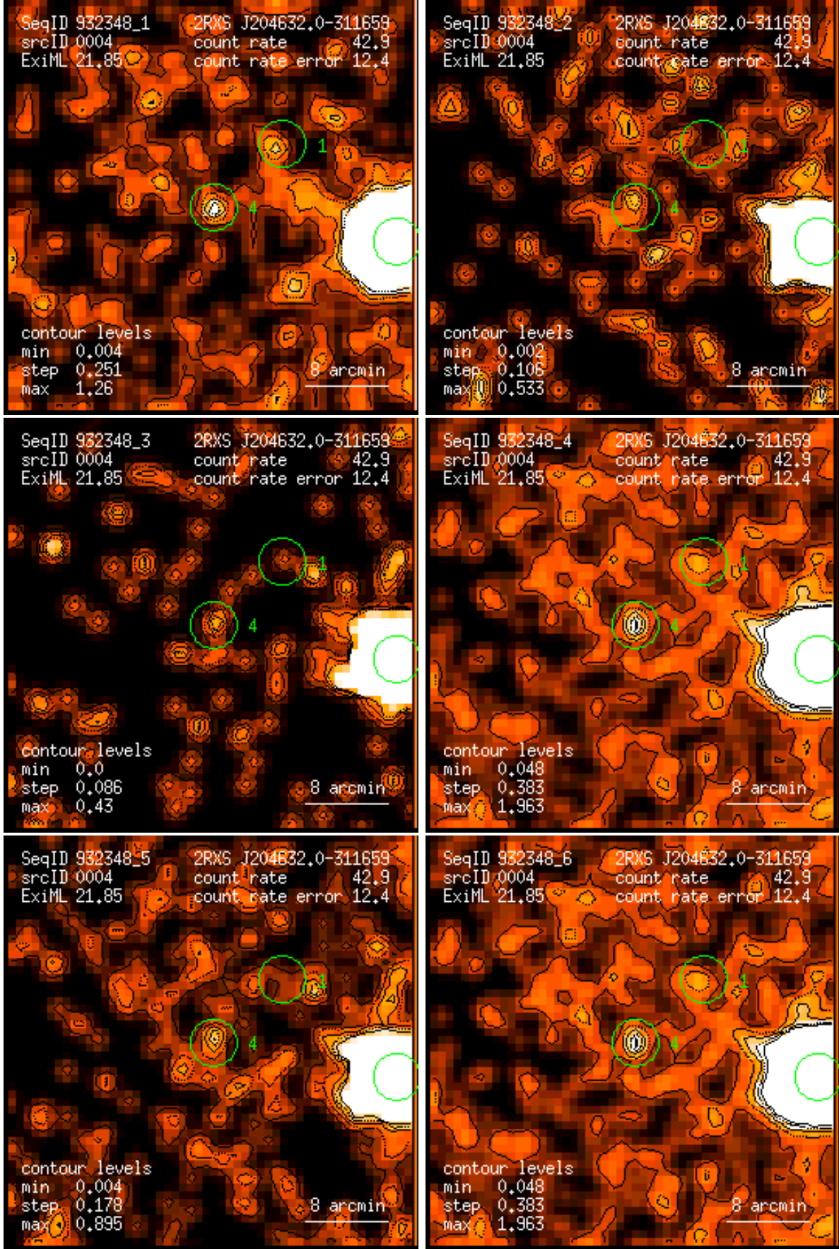
Figure 4: RASS 932348: detection 0004: band rate images, Gaussian filter: (1) PSPC channels 11 – 41, (2) 52 – 90, (3) 91 – 201, (4) 11 – 235, (5) 52 – 201, (6) 11 – 201. Broad band rates in counts/ks. Band rate contour levels in counts/ks/arcmin 2 .
