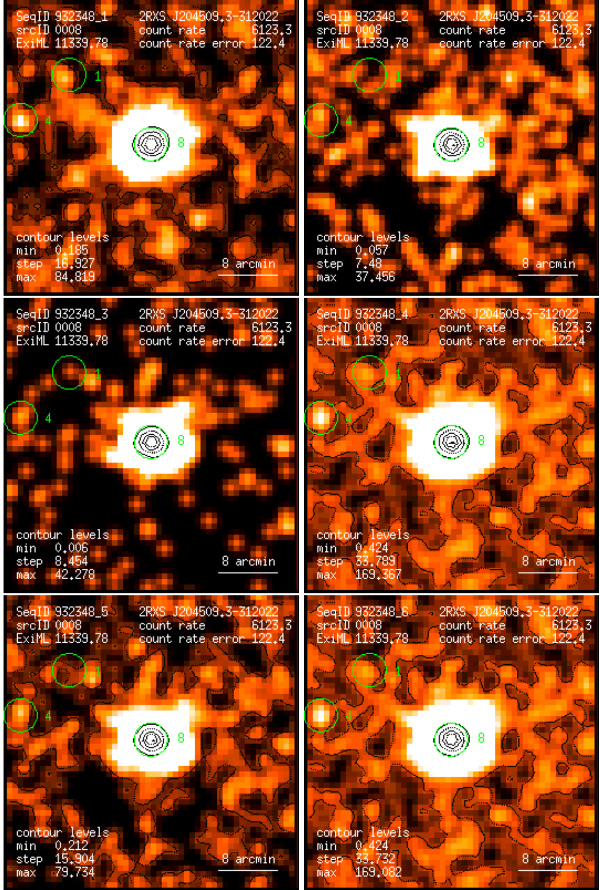
Figure 8: RASS 932348: detection 0008: band rate images, Gaussian filter: (1) PSPC channels 11 – 41, (2) 52 – 90, (3) 91 – 201, (4) 11 – 235, (5) 52 – 201, (6) 11 – 201. Broad band rates in counts/ks. Band rate contour levels in counts/ks/arcmin 2 .
