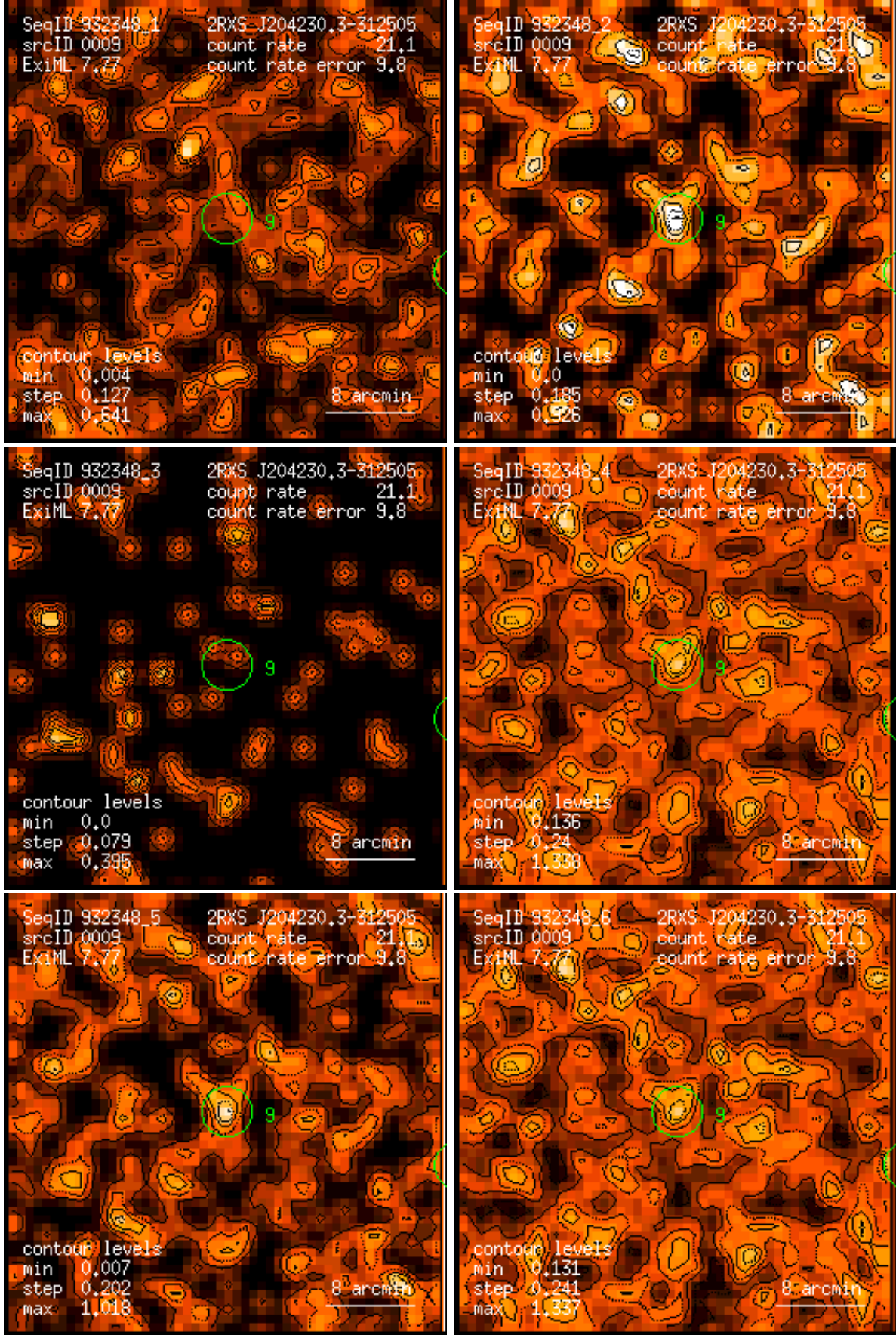
Figure 9: RASS 932348: detection 0009: band rate images, Gaussian filter: (1) PSPC channels 11 – 41, (2) 52 – 90, (3) 91 – 201, (4) 11 – 235, (5) 52 – 201, (6) 11 – 201. Broad band rates in counts/ks. Band rate contour levels in counts/ks/arcmin 2 .
