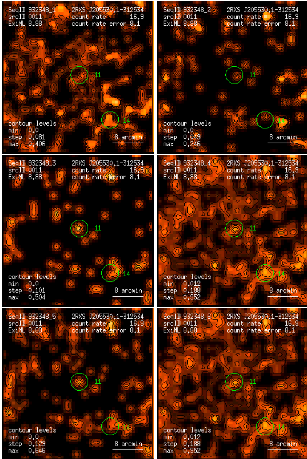
Figure 11: RASS 932348: detection 0011: band rate images, Gaussian filter: (1) PSPC channels 11 – 41, (2) 52 – 90, (3) 91 – 201, (4) 11 – 235, (5) 52 – 201, (6) 11 – 201. Broad band rates in counts/ks. Band rate contour levels in counts/ks/arcmin 2 .
