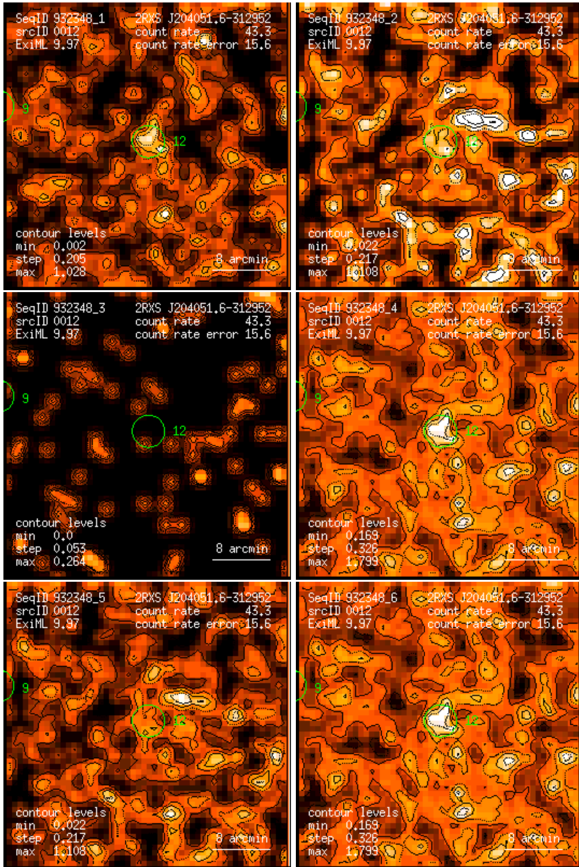
Figure 12: RASS 932348: detection 0012: band rate images, Gaussian filter: (1) PSPC channels 11 – 41, (2) 52 – 90, (3) 91 – 201, (4) 11 – 235, (5) 52 – 201, (6) 11 – 201. Broad band rates in counts/ks. Band rate contour levels in counts/ks/arcmin 2 .
