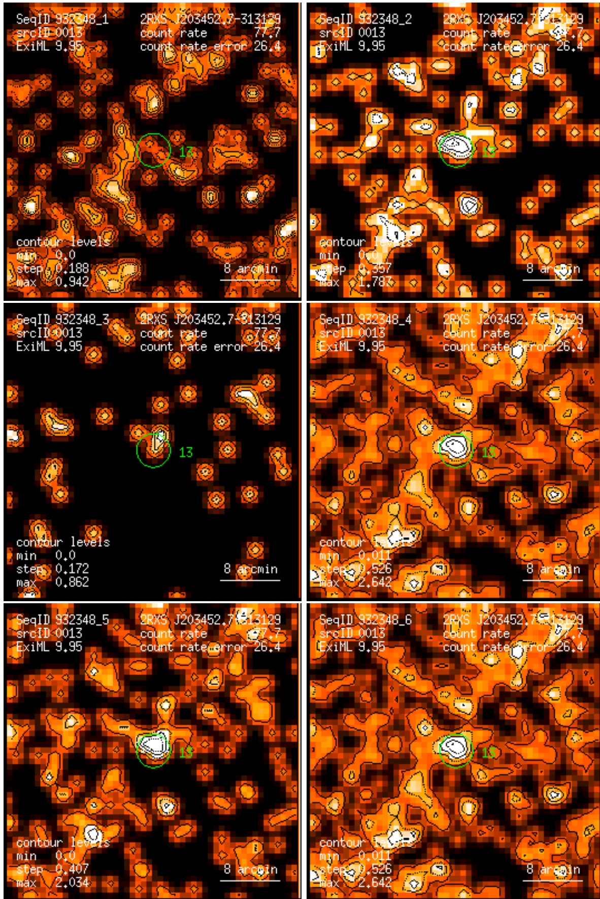
Figure 13: RASS 932348: detection 0013: band rate images, Gaussian filter: (1) PSPC channels 11 – 41, (2) 52 – 90, (3) 91 – 201, (4) 11 – 235, (5) 52 – 201, (6) 11 – 201. Broad band rates in counts/ks. Band rate contour levels in counts/ks/arcmin 2 .
