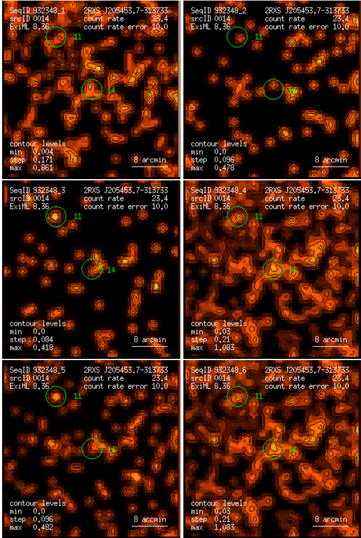
Figure 14: RASS 932348: detection 0014: band rate images, Gaussian filter: (1) PSPC channels 11 – 41, (2) 52 – 90, (3) 91 – 201, (4) 11 – 235, (5) 52 – 201, (6) 11 – 201. Broad band rates in counts/ks. Band rate contour levels in counts/ks/arcmin 2 .
