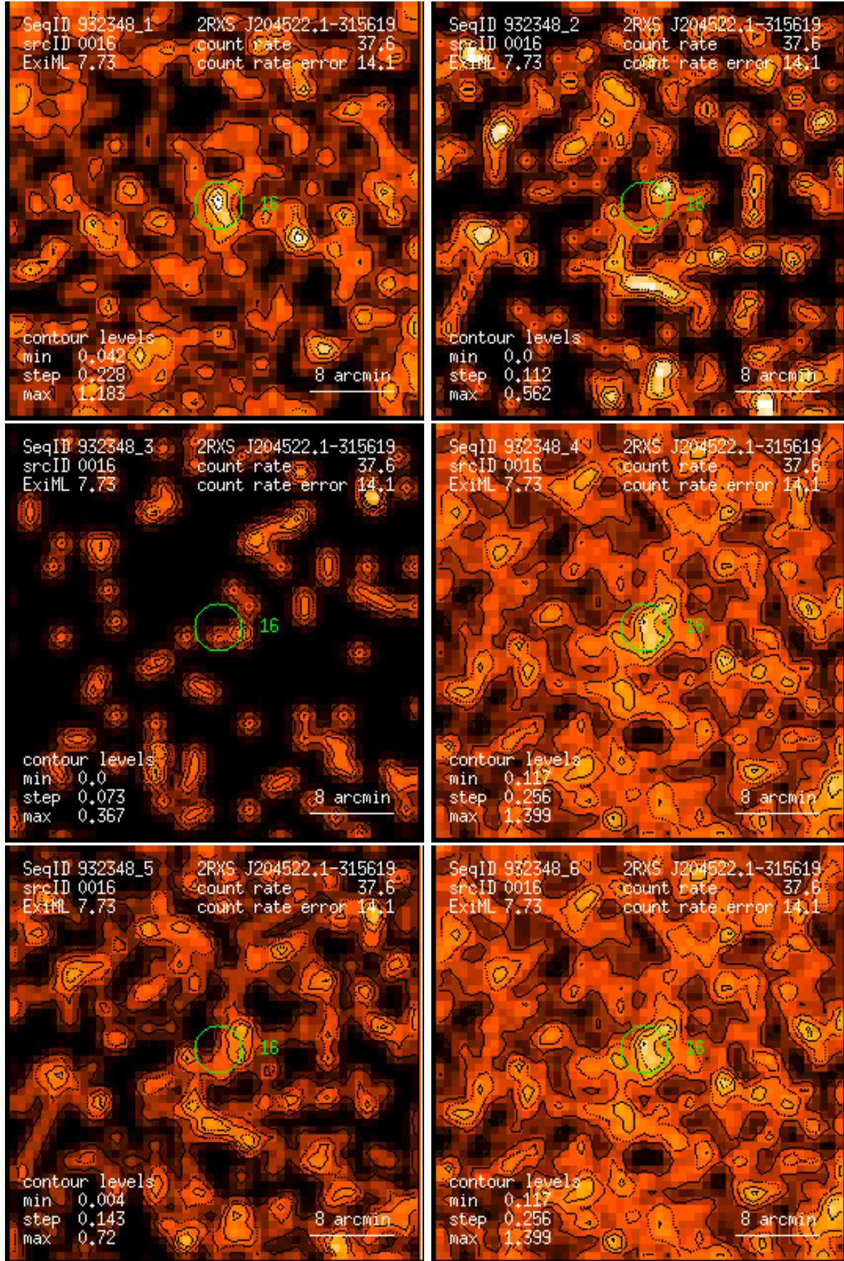
Figure 16: RASS 932348: detection 0016: band rate images, Gaussian filter: (1) PSPC channels 11 – 41, (2) 52 – 90, (3) 91 – 201, (4) 11 – 235, (5) 52 – 201, (6) 11 – 201. Broad band rates in counts/ks. Band rate contour levels in counts/ks/arcmin 2 .
