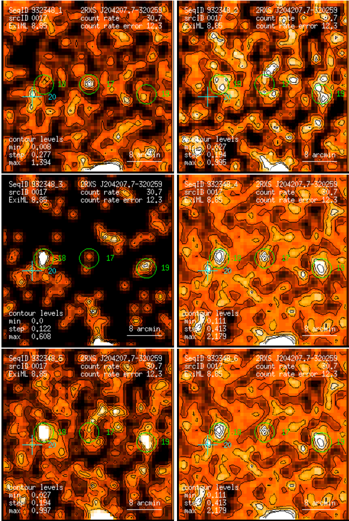
Figure 17: RASS 932348: detection 0017: band rate images, Gaussian filter: (1) PSPC channels 11 – 41, (2) 52 – 90, (3) 91 – 201, (4) 11 – 235, (5) 52 – 201, (6) 11 – 201. Broad band rates in counts/ks. Band rate contour levels in counts/ks/arcmin 2 .
