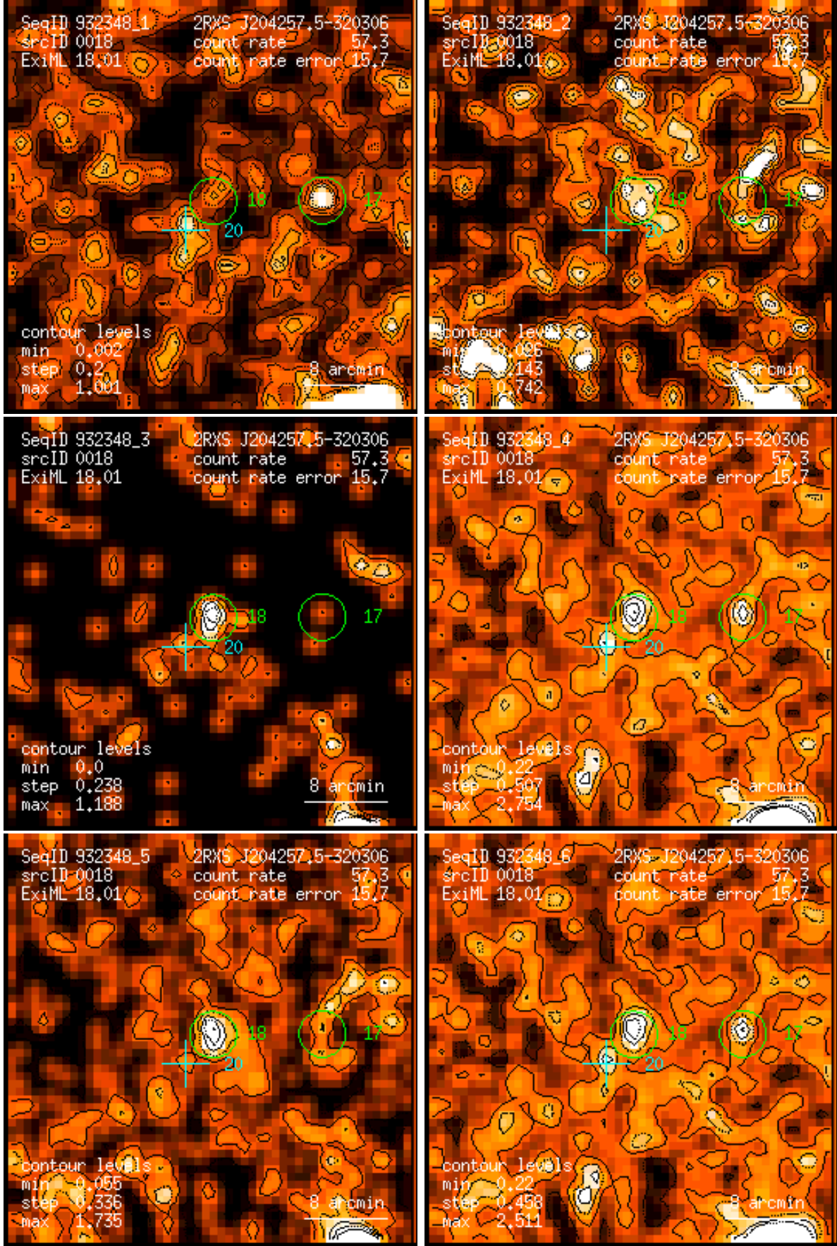
Figure 18: RASS 932348: detection 0018: band rate images, Gaussian filter: (1) PSPC channels 11 – 41, (2) 52 – 90, (3) 91 – 201, (4) 11 – 235, (5) 52 – 201, (6) 11 – 201. Broad band rates in counts/ks. Band rate contour levels in counts/ks/arcmin 2 .
