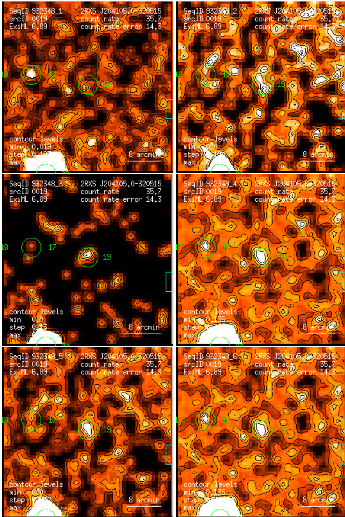
Figure 19: RASS 932348: detection 0019: band rate images, Gaussian filter: (1) PSPC channels 11 – 41, (2) 52 – 90, (3) 91 – 201, (4) 11 – 235, (5) 52 – 201, (6) 11 – 201. Broad band rates in counts/ks. Band rate contour levels in counts/ks/arcmin 2 .
