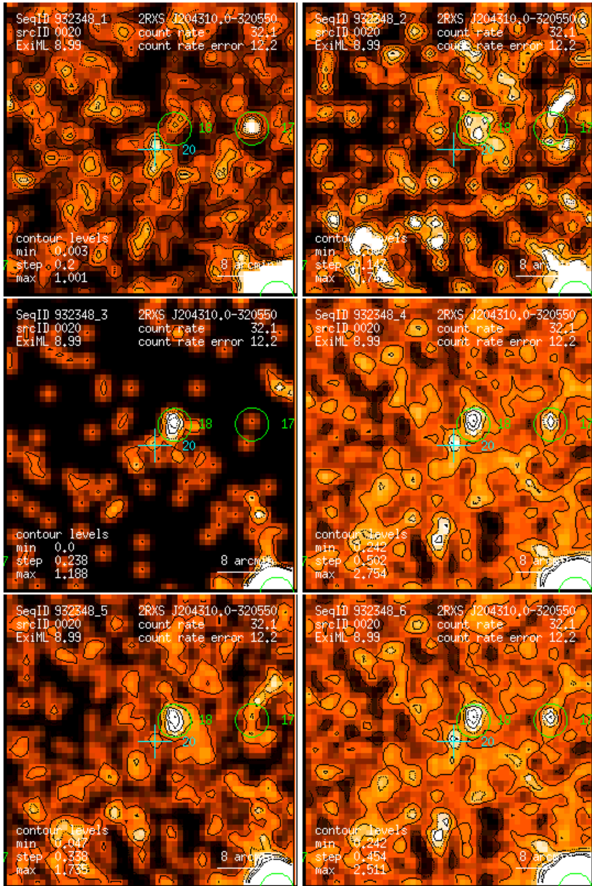
Figure 20: RASS 932348: detection 0020: band rate images, Gaussian filter: (1) PSPC channels 11 – 41, (2) 52 – 90, (3) 91 – 201, (4) 11 – 235, (5) 52 – 201, (6) 11 – 201. Broad band rates in counts/ks. Band rate contour levels in counts/ks/arcmin 2 .
