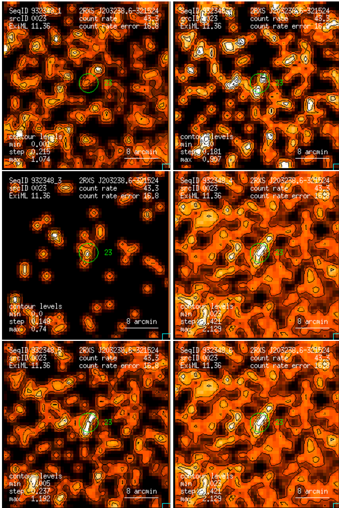
Figure 23: RASS 932348: detection 0023: band rate images, Gaussian filter: (1) PSPC channels 11 – 41, (2) 52 – 90, (3) 91 – 201, (4) 11 – 235, (5) 52 – 201, (6) 11 – 201. Broad band rates in counts/ks. Band rate contour levels in counts/ks/arcmin 2 .
