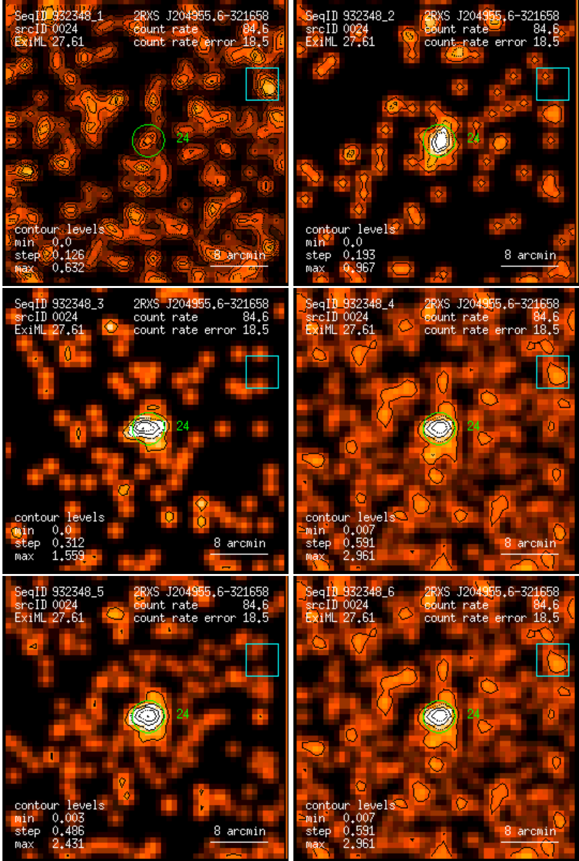
Figure 24: RASS 932348: detection 0024: band rate images, Gaussian filter: (1) PSPC channels 11 – 41, (2) 52 – 90, (3) 91 – 201, (4) 11 – 235, (5) 52 – 201, (6) 11 – 201. Broad band rates in counts/ks. Band rate contour levels in counts/ks/arcmin 2 .
