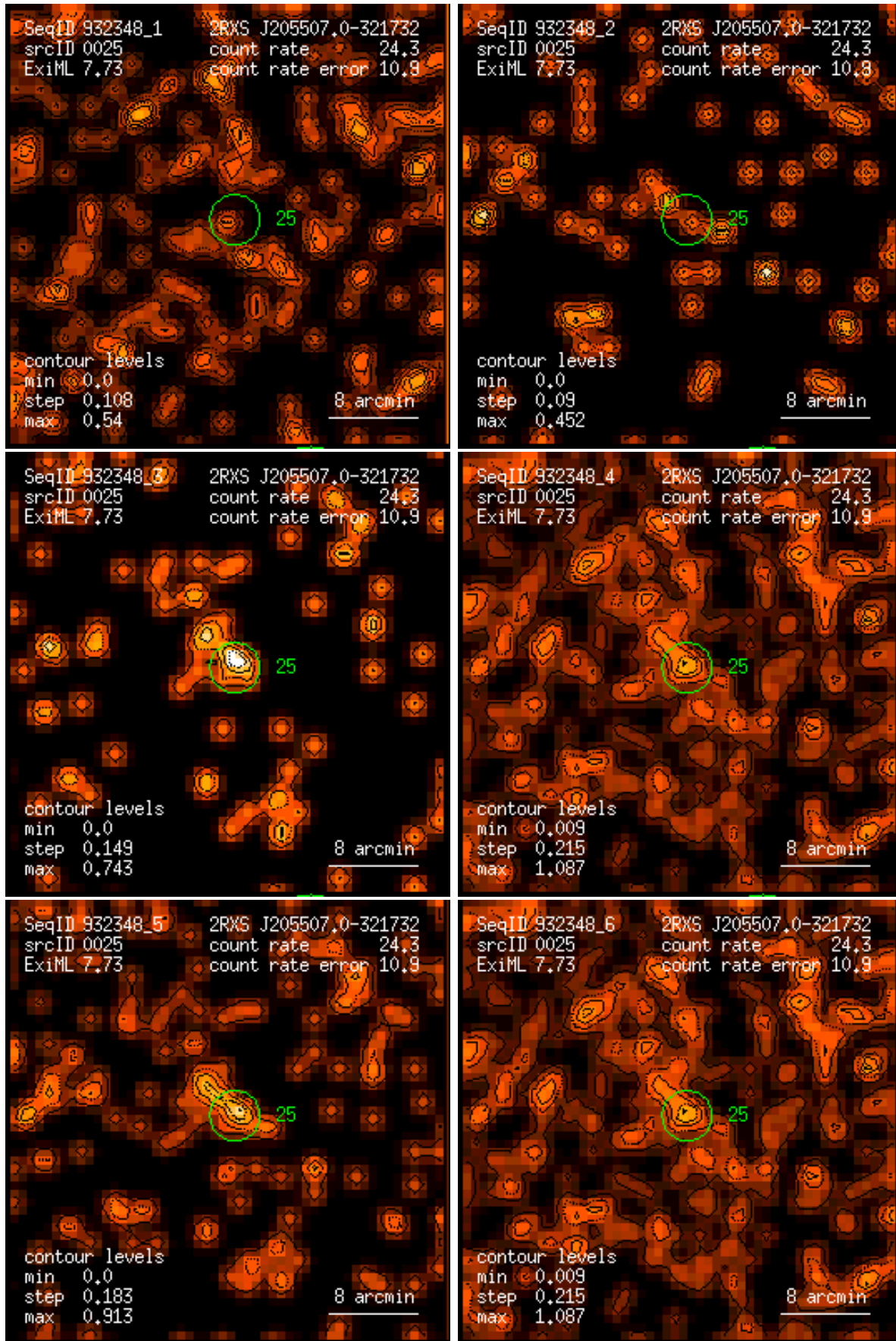
Figure 25: RASS 932348: detection 0025: band rate images, Gaussian filter: (1) PSPC channels 11 – 41, (2) 52 – 90, (3) 91 – 201, (4) 11 – 235, (5) 52 – 201, (6) 11 – 201. Broad band rates in counts/ks. Band rate contour levels in counts/ks/arcmin 2 .
