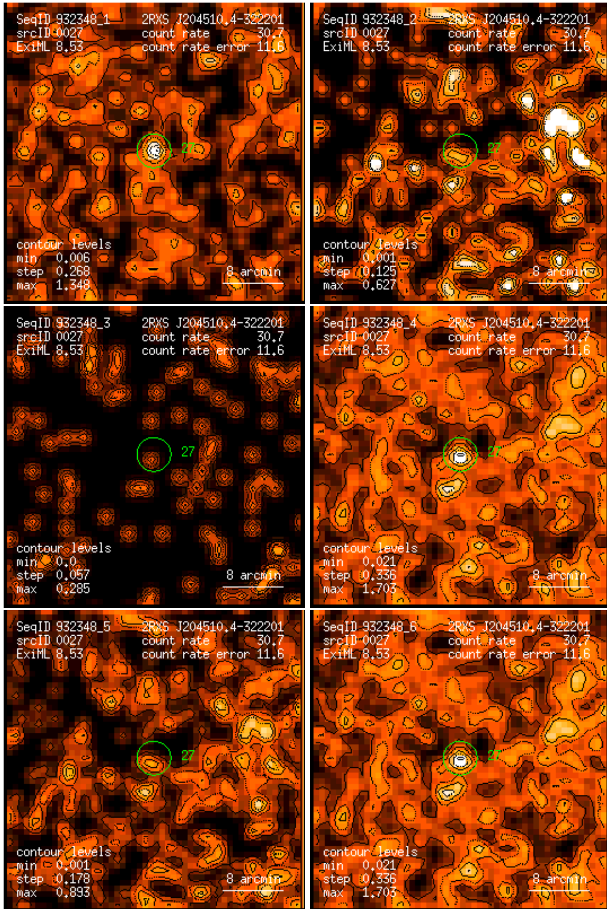
Figure 27: RASS 932348: detection 0027: band rate images, Gaussian filter: (1) PSPC channels 11 – 41, (2) 52 – 90, (3) 91 – 201, (4) 11 – 235, (5) 52 – 201, (6) 11 – 201. Broad band rates in counts/ks. Band rate contour levels in counts/ks/arcmin 2 .
