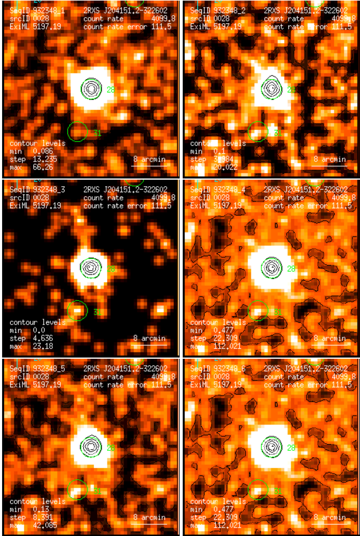
Figure 28: RASS 932348: detection 0028: band rate images, Gaussian filter: (1) PSPC channels 11 – 41, (2) 52 – 90, (3) 91 – 201, (4) 11 – 235, (5) 52 – 201, (6) 11 – 201. Broad band rates in counts/ks. Band rate contour levels in counts/ks/arcmin 2 .
