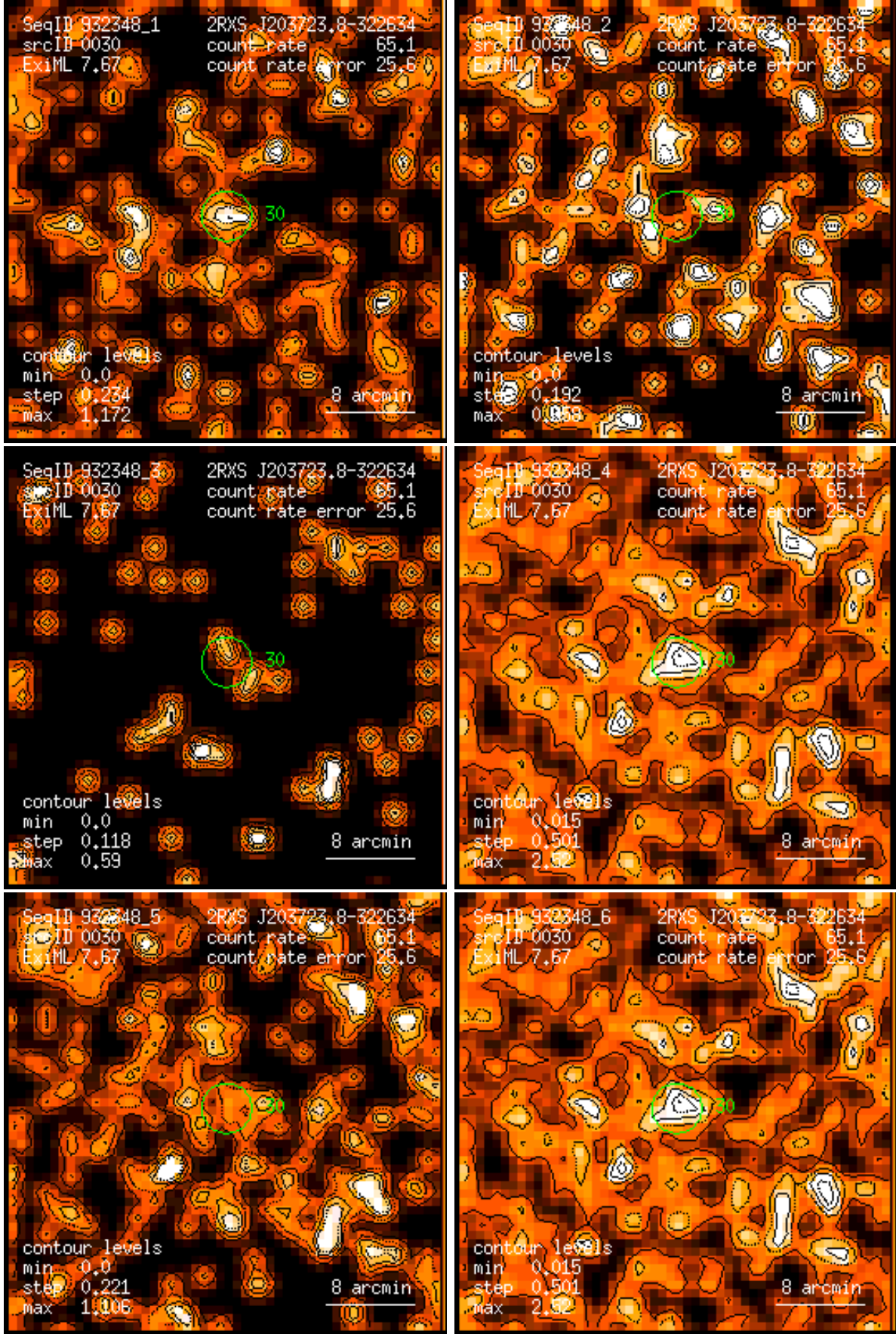
Figure 30: RASS 932348: detection 0030: band rate images, Gaussian filter: (1) PSPC channels 11 – 41, (2) 52 – 90, (3) 91 – 201, (4) 11 – 235, (5) 52 – 201, (6) 11 – 201. Broad band rates in counts/ks. Band rate contour levels in counts/ks/arcmin 2 .
