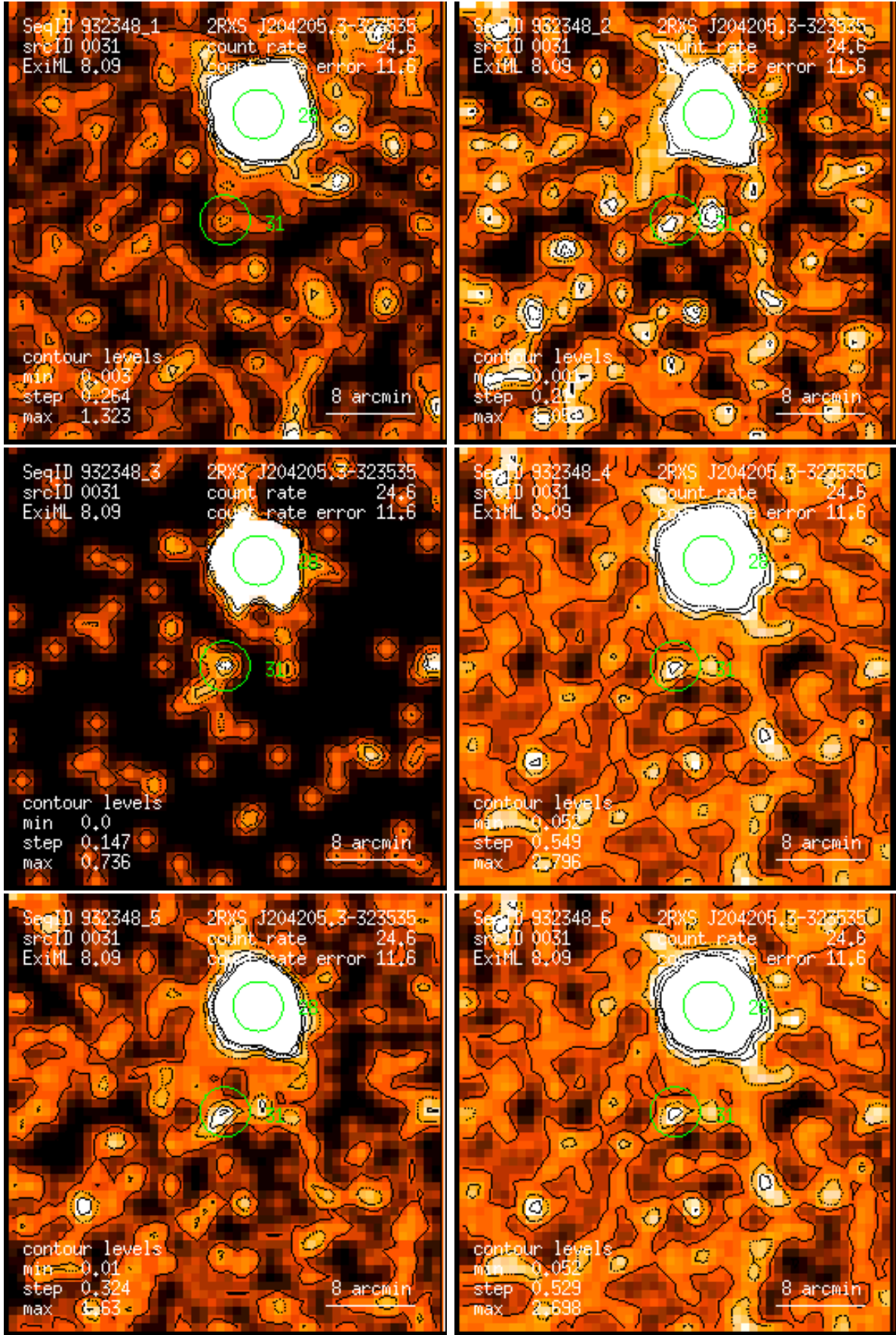
Figure 31: RASS 932348: detection 0031: band rate images, Gaussian filter: (1) PSPC channels 11 – 41, (2) 52 – 90, (3) 91 – 201, (4) 11 – 235, (5) 52 – 201, (6) 11 – 201. Broad band rates in counts/ks. Band rate contour levels in counts/ks/arcmin 2 .
