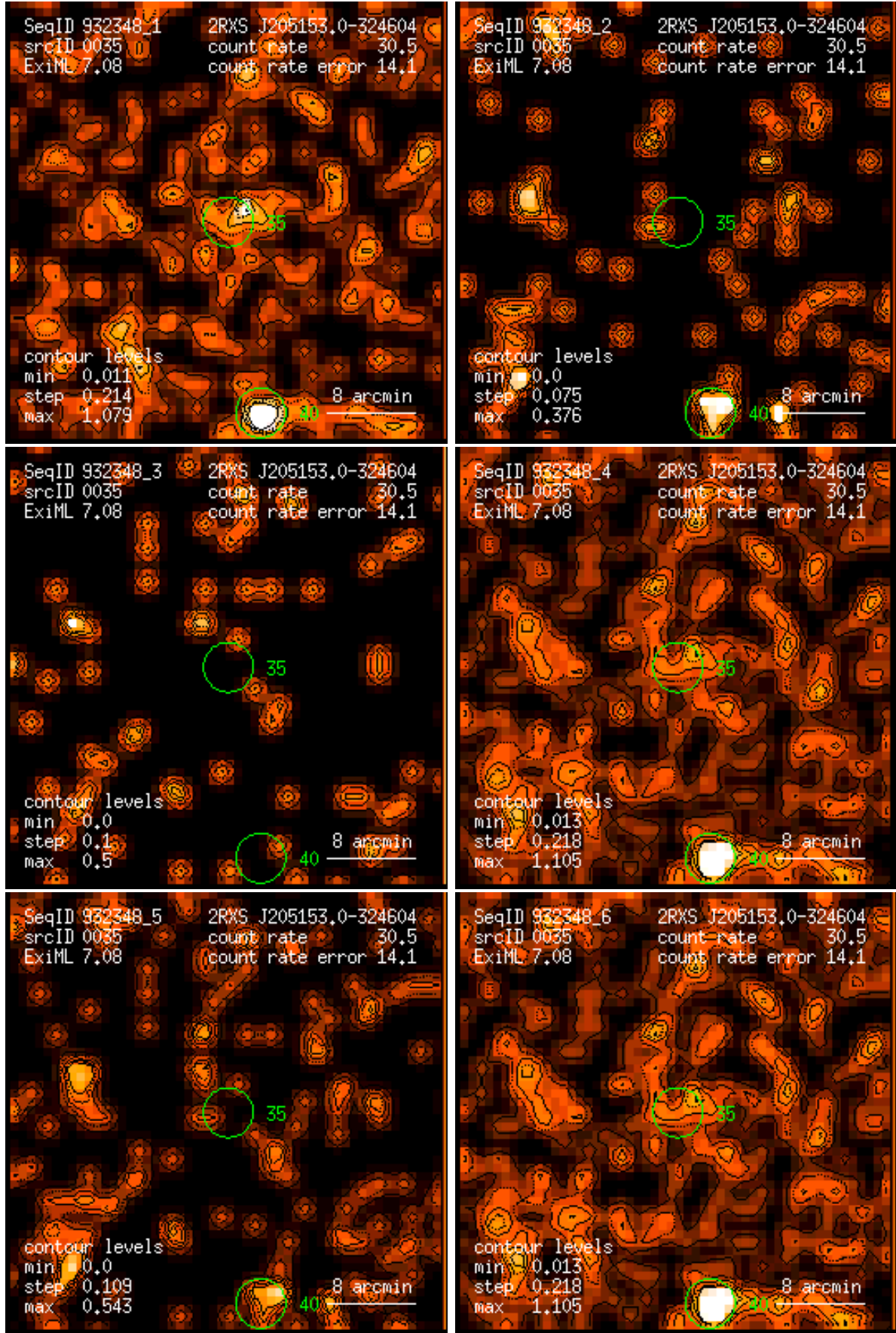
Figure 35: RASS 932348: detection 0035: band rate images, Gaussian filter: (1) PSPC channels 11 – 41, (2) 52 – 90, (3) 91 – 201, (4) 11 – 235, (5) 52 – 201, (6) 11 – 201. Broad band rates in counts/ks. Band rate contour levels in counts/ks/arcmin 2 .
