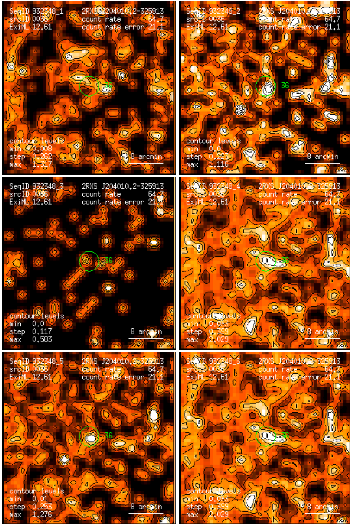
Figure 36: RASS 932348: detection 0036: band rate images, Gaussian filter: (1) PSPC channels 11 – 41, (2) 52 – 90, (3) 91 – 201, (4) 11 – 235, (5) 52 – 201, (6) 11 – 201. Broad band rates in counts/ks. Band rate contour levels in counts/ks/arcmin 2 .
