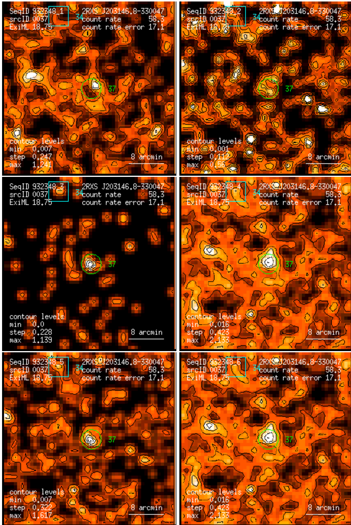
Figure 37: RASS 932348: detection 0037: band rate images, Gaussian filter: (1) PSPC channels 11 – 41, (2) 52 – 90, (3) 91 – 201, (4) 11 – 235, (5) 52 – 201, (6) 11 – 201. Broad band rates in counts/ks. Band rate contour levels in counts/ks/arcmin 2 .
