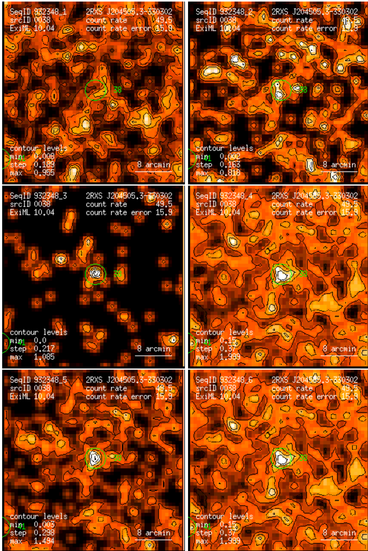
Figure 38: RASS 932348: detection 0038: band rate images, Gaussian filter: (1) PSPC channels 11 – 41, (2) 52 – 90, (3) 91 – 201, (4) 11 – 235, (5) 52 – 201, (6) 11 – 201. Broad band rates in counts/ks. Band rate contour levels in counts/ks/arcmin 2 .
