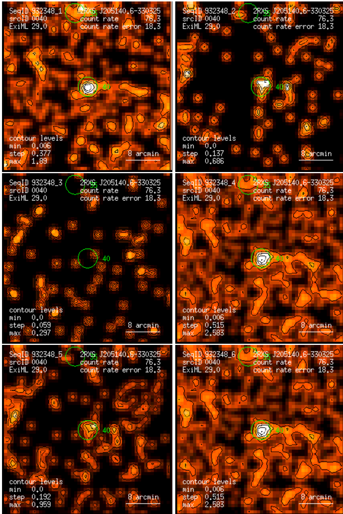
Figure 40: RASS 932348: detection 0040: band rate images, Gaussian filter: (1) PSPC channels 11 – 41, (2) 52 – 90, (3) 91 – 201, (4) 11 – 235, (5) 52 – 201, (6) 11 – 201. Broad band rates in counts/ks. Band rate contour levels in counts/ks/arcmin 2 .
