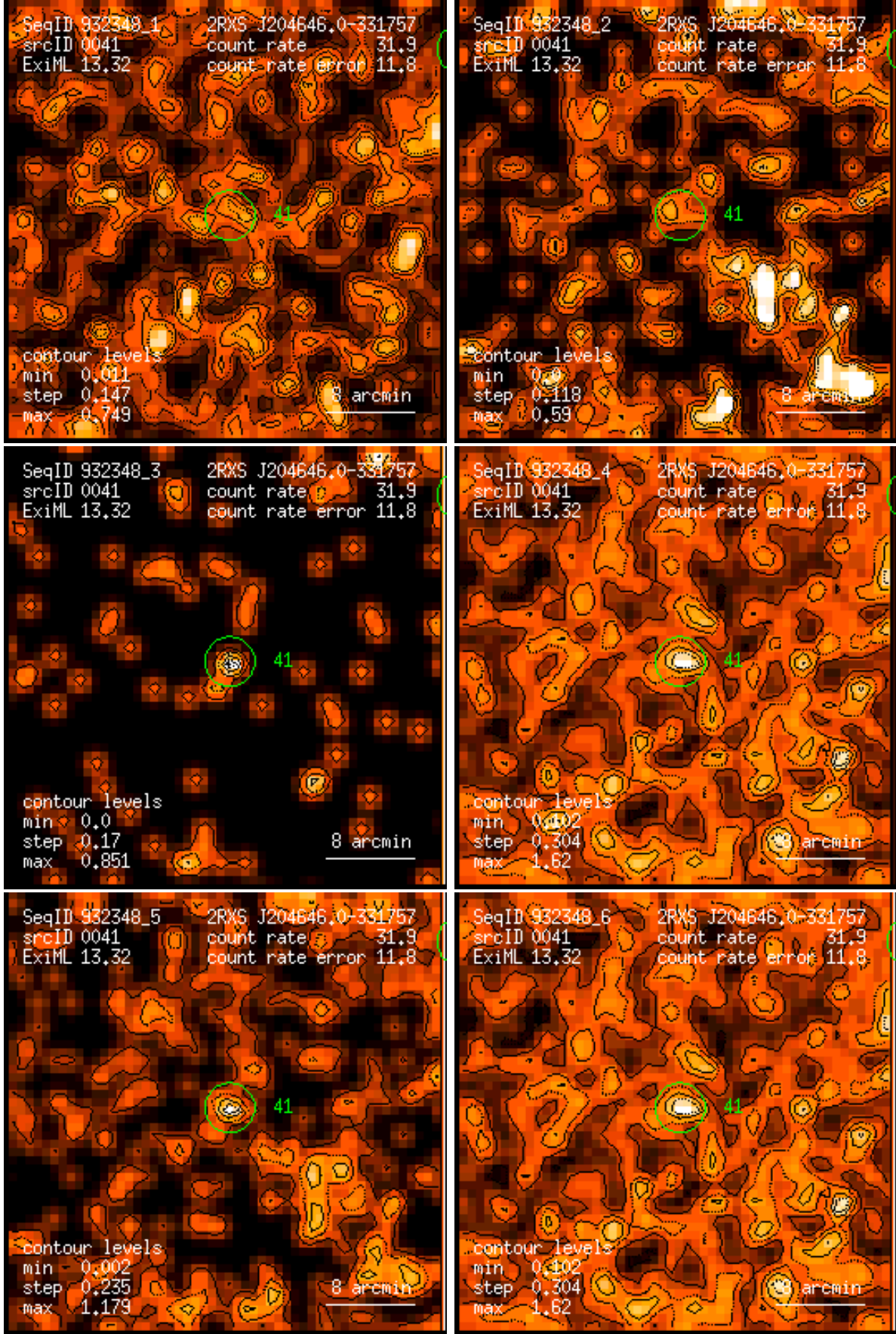
Figure 41: RASS 932348: detection 0041: band rate images, Gaussian filter: (1) PSPC channels 11 – 41, (2) 52 – 90, (3) 91 – 201, (4) 11 – 235, (5) 52 – 201, (6) 11 – 201. Broad band rates in counts/ks. Band rate contour levels in counts/ks/arcmin 2 .
