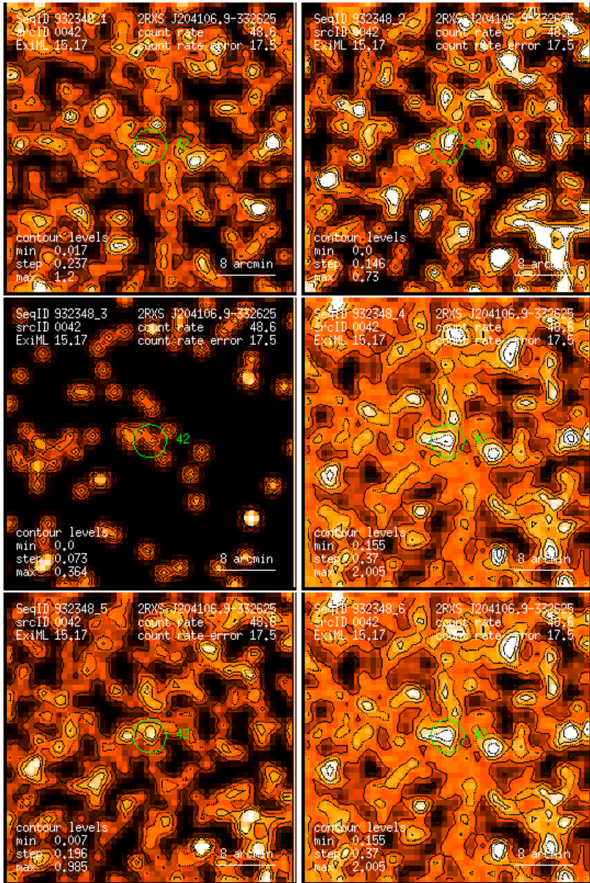
Figure 42: RASS 932348: detection 0042: band rate images, Gaussian filter: (1) PSPC channels 11 – 41, (2) 52 – 90, (3) 91 – 201, (4) 11 – 235, (5) 52 – 201, (6) 11 – 201. Broad band rates in counts/ks. Band rate contour levels in counts/ks/arcmin 2 .
