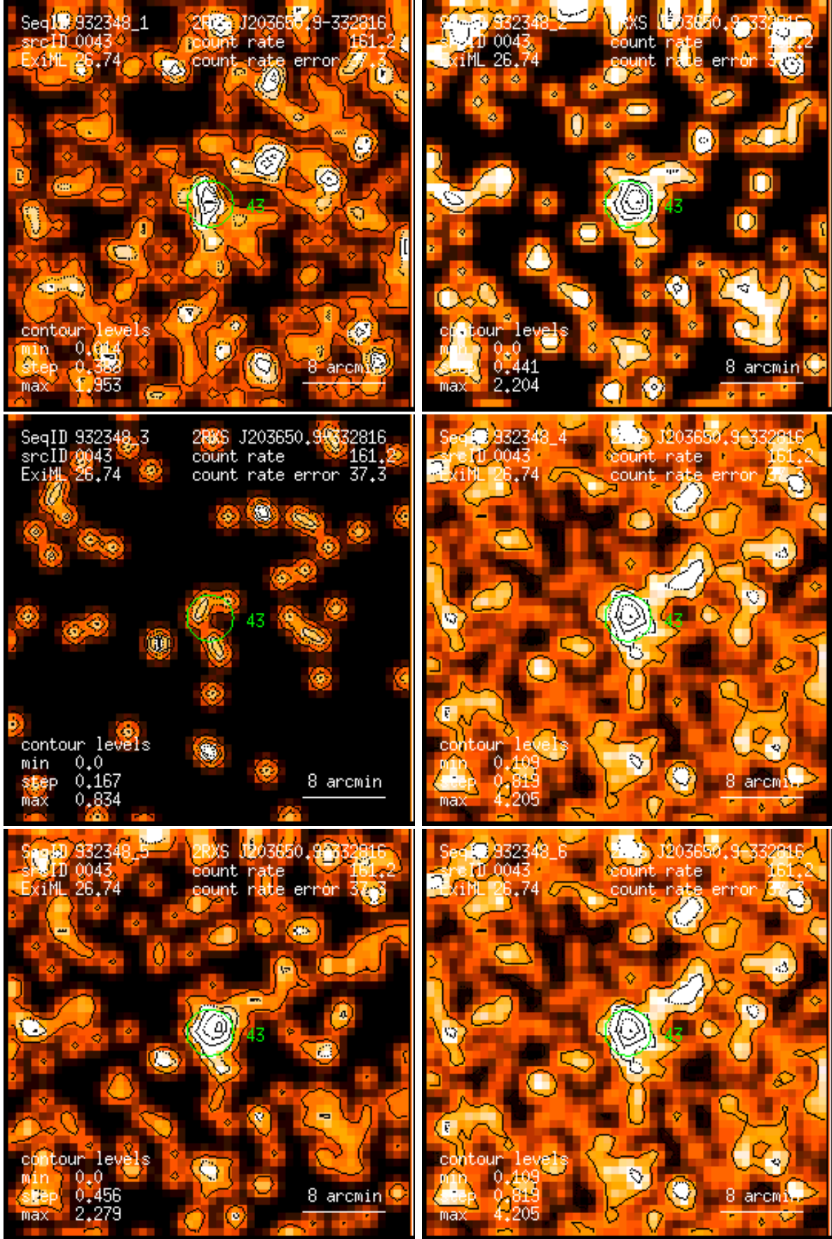
Figure 43: RASS 932348: detection 0043: band rate images, Gaussian filter: (1) PSPC channels 11 – 41, (2) 52 – 90, (3) 91 – 201, (4) 11 – 235, (5) 52 – 201, (6) 11 – 201. Broad band rates in counts/ks. Band rate contour levels in counts/ks/arcmin 2 .
