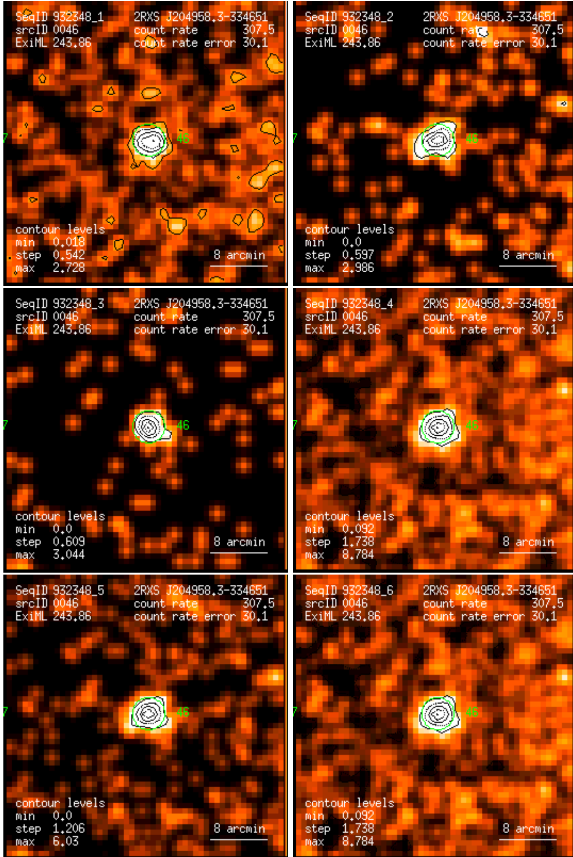
Figure 46: RASS 932348: detection 0046: band rate images, Gaussian filter: (1) PSPC channels 11 – 41, (2) 52 – 90, (3) 91 – 201, (4) 11 – 235, (5) 52 – 201, (6) 11 – 201. Broad band rates in counts/ks. Band rate contour levels in counts/ks/arcmin 2 .
