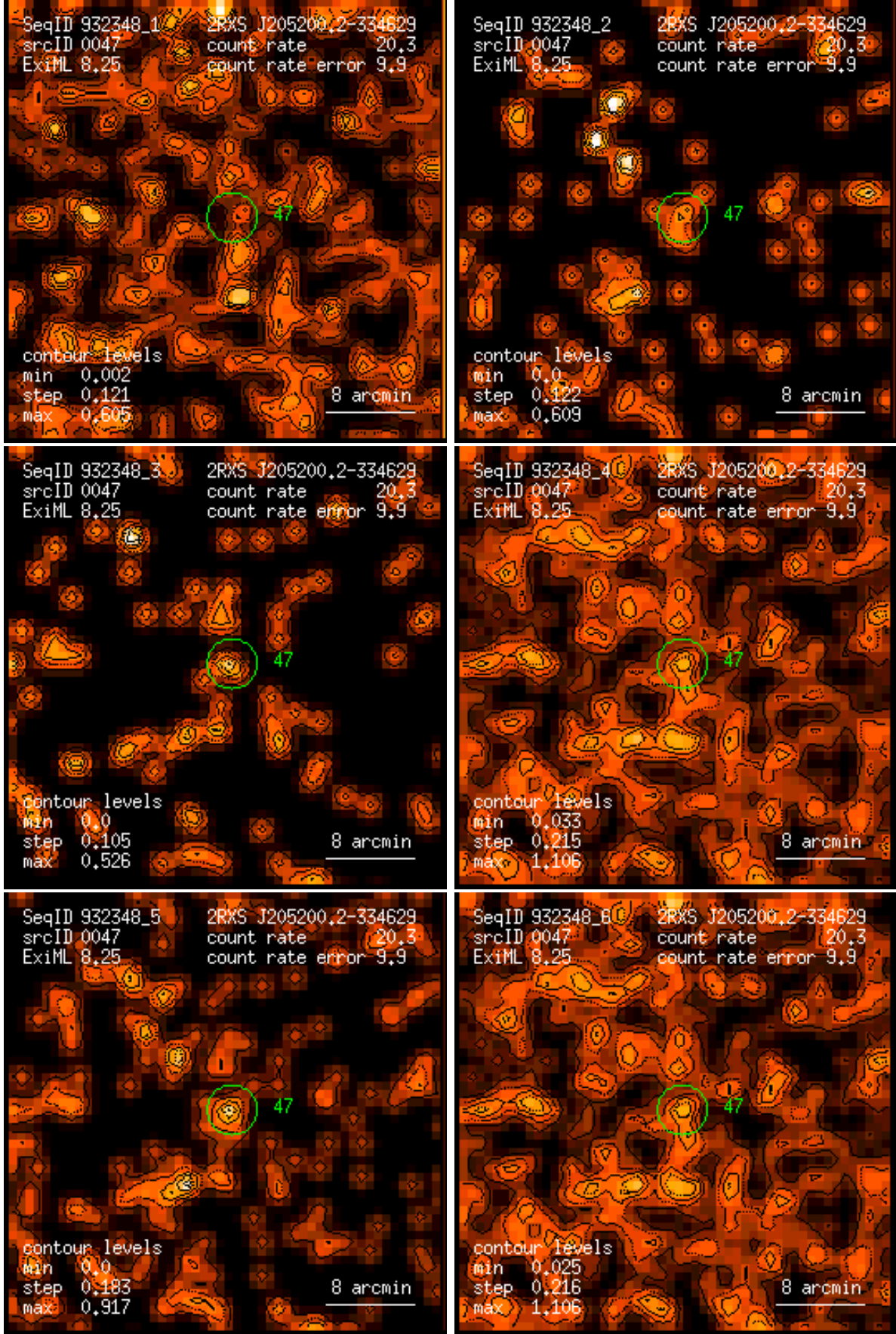
Figure 47: RASS 932348: detection 0047: band rate images, Gaussian filter: (1) PSPC channels 11 – 41, (2) 52 – 90, (3) 91 – 201, (4) 11 – 235, (5) 52 – 201, (6) 11 – 201. Broad band rates in counts/ks. Band rate contour levels in counts/ks/arcmin 2 .
