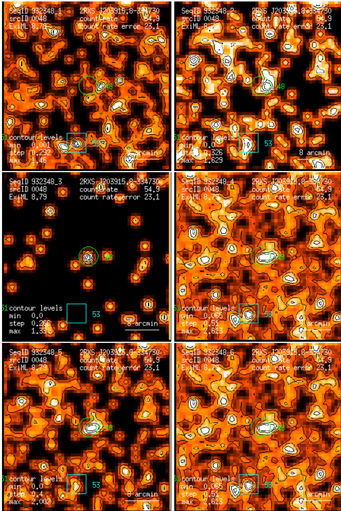
Figure 48: RASS 932348: detection 0048: band rate images, Gaussian filter: (1) PSPC channels 11 – 41, (2) 52 – 90, (3) 91 – 201, (4) 11 – 235, (5) 52 – 201, (6) 11 – 201. Broad band rates in counts/ks. Band rate contour levels in counts/ks/arcmin 2 .
