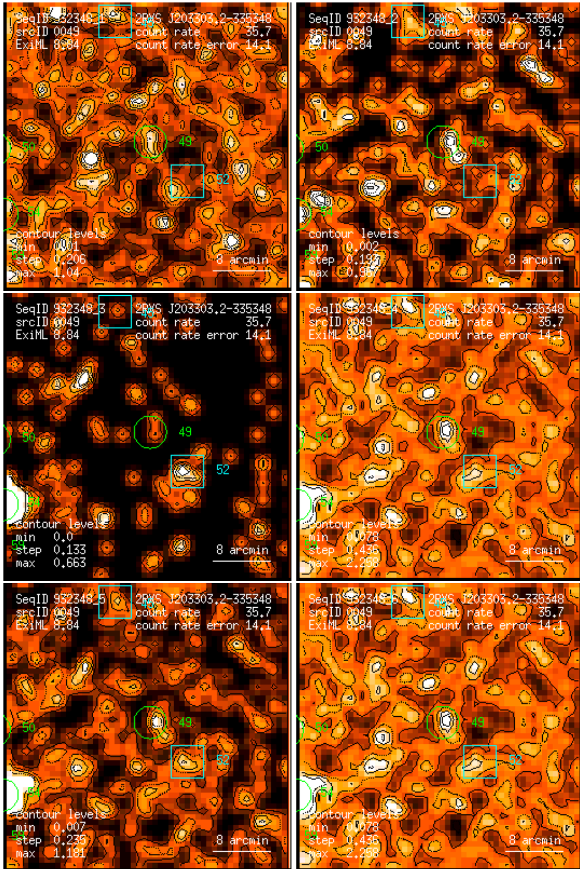
Figure 49: RASS 932348: detection 0049: band rate images, Gaussian filter: (1) PSPC channels 11 – 41, (2) 52 – 90, (3) 91 – 201, (4) 11 – 235, (5) 52 – 201, (6) 11 – 201. Broad band rates in counts/ks. Band rate contour levels in counts/ks/arcmin 2 .
