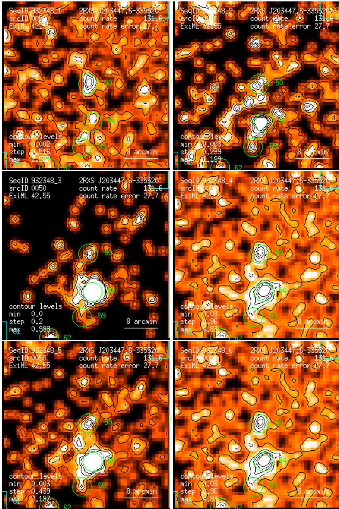
Figure 50: RASS 932348: detection 0050: band rate images, Gaussian filter: (1) PSPC channels 11 – 41, (2) 52 – 90, (3) 91 – 201, (4) 11 – 235, (5) 52 – 201, (6) 11 – 201. Broad band rates in counts/ks. Band rate contour levels in counts/ks/arcmin 2 .
