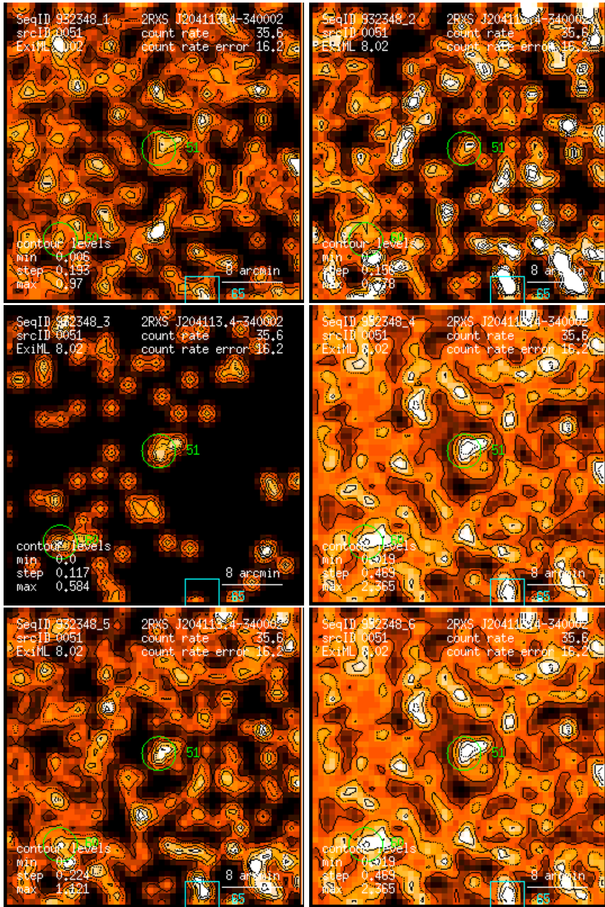
Figure 51: RASS 932348: detection 0051: band rate images, Gaussian filter: (1) PSPC channels 11 – 41, (2) 52 – 90, (3) 91 – 201, (4) 11 – 235, (5) 52 – 201, (6) 11 – 201. Broad band rates in counts/ks. Band rate contour levels in counts/ks/arcmin 2 .
