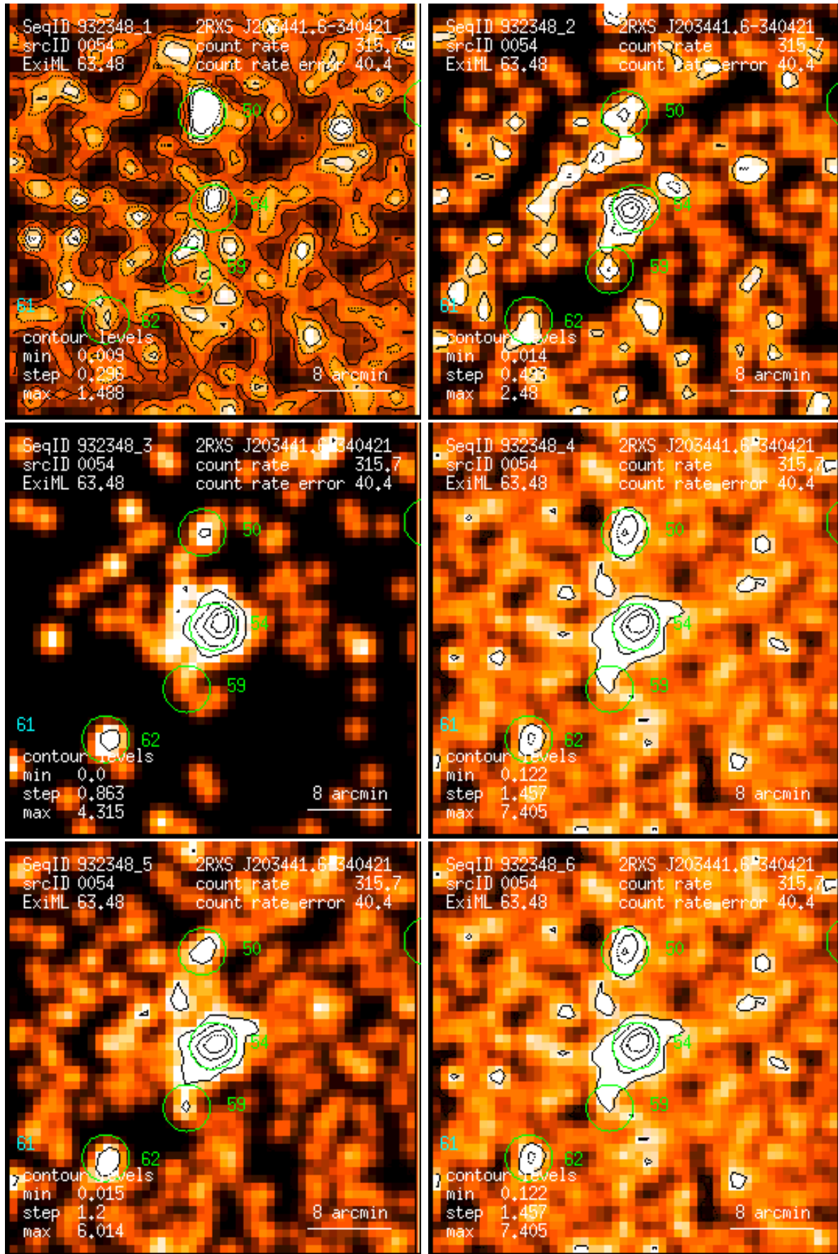
Figure 54: RASS 932348: detection 0054: band rate images, Gaussian filter: (1) PSPC channels 11 – 41, (2) 52 – 90, (3) 91 – 201, (4) 11 – 235, (5) 52 – 201, (6) 11 – 201. Broad band rates in counts/ks. Band rate contour levels in counts/ks/arcmin 2 .
