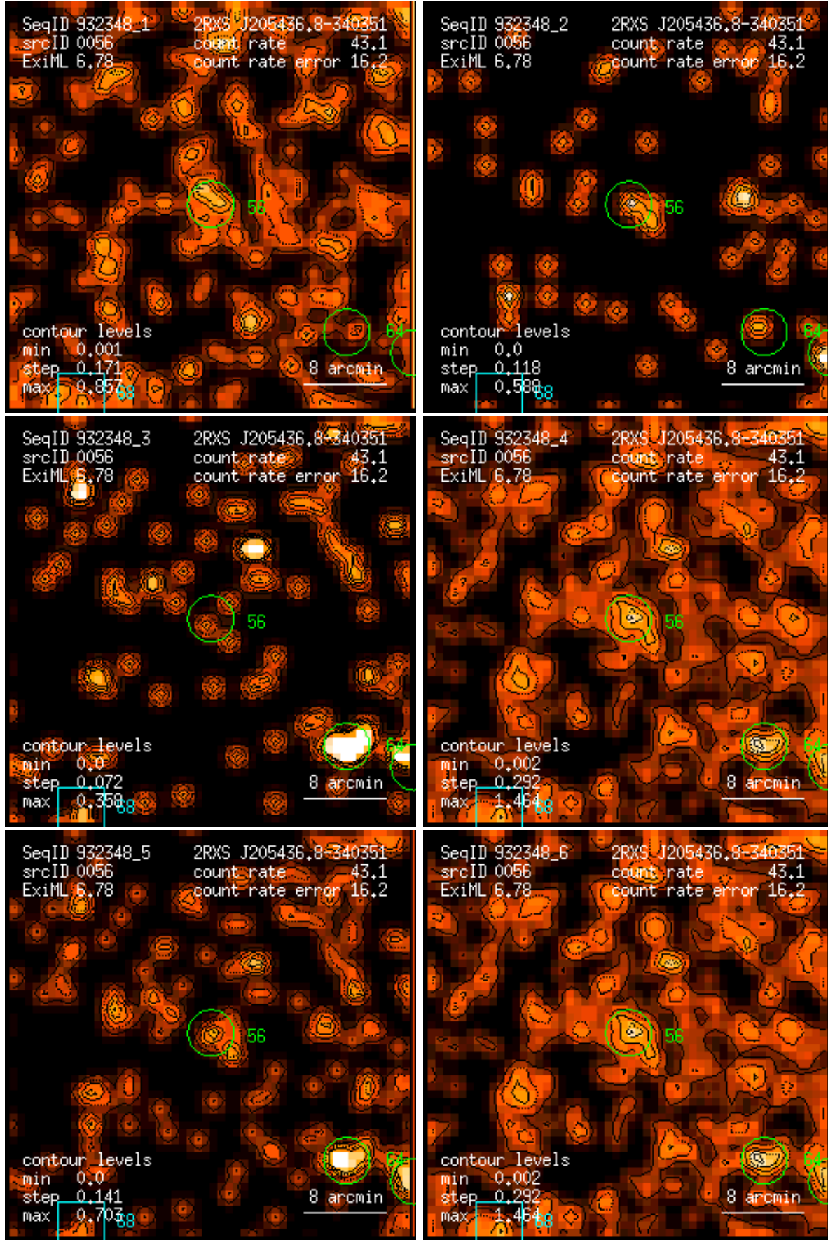
Figure 56: RASS 932348: detection 0056: band rate images, Gaussian filter: (1) PSPC channels 11 – 41, (2) 52 – 90, (3) 91 – 201, (4) 11 – 235, (5) 52 – 201, (6) 11 – 201. Broad band rates in counts/ks. Band rate contour levels in counts/ks/arcmin 2 .
