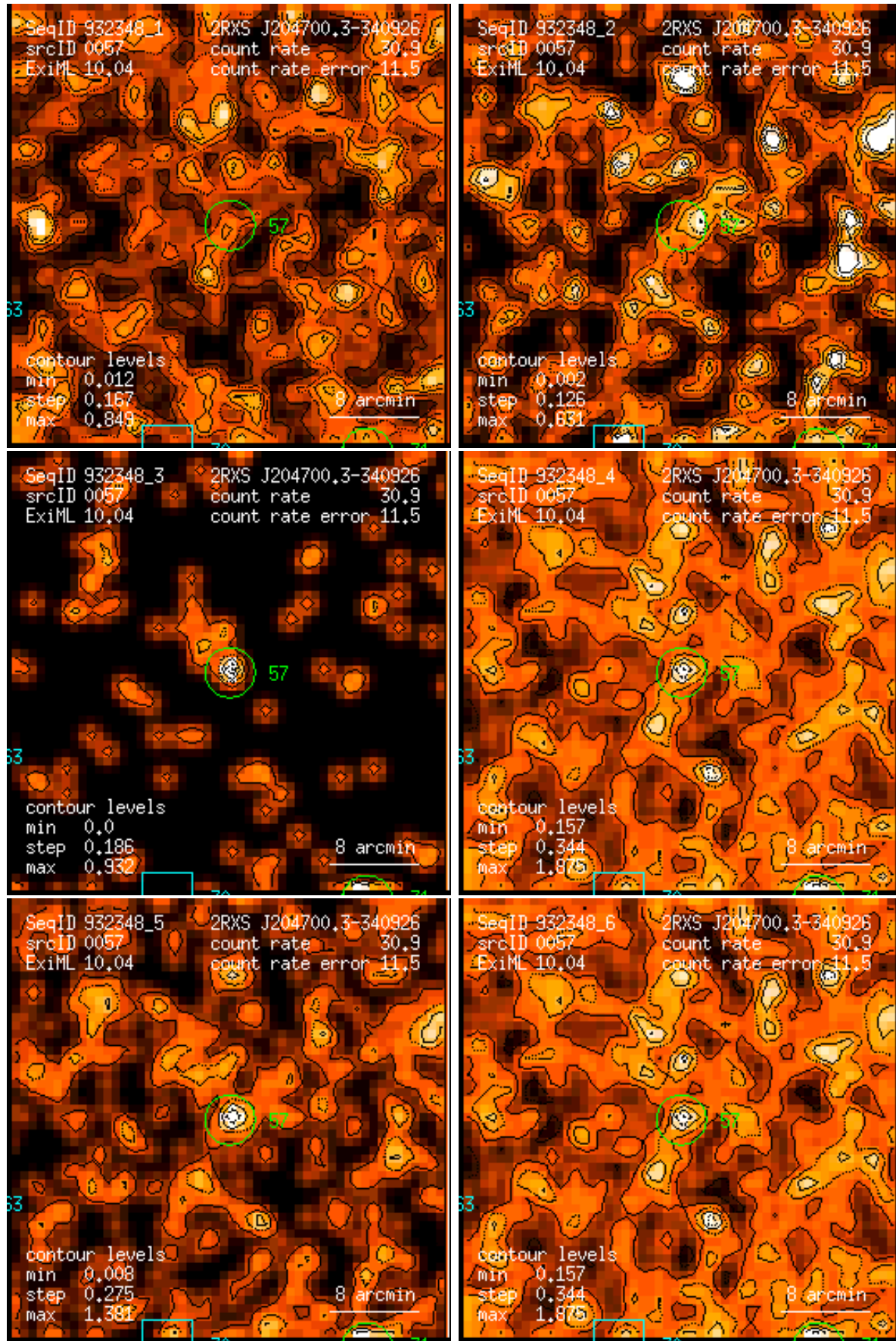
Figure 57: RASS 932348: detection 0057: band rate images, Gaussian filter: (1) PSPC channels 11 – 41, (2) 52 – 90, (3) 91 – 201, (4) 11 – 235, (5) 52 – 201, (6) 11 – 201. Broad band rates in counts/ks. Band rate contour levels in counts/ks/arcmin 2 .
