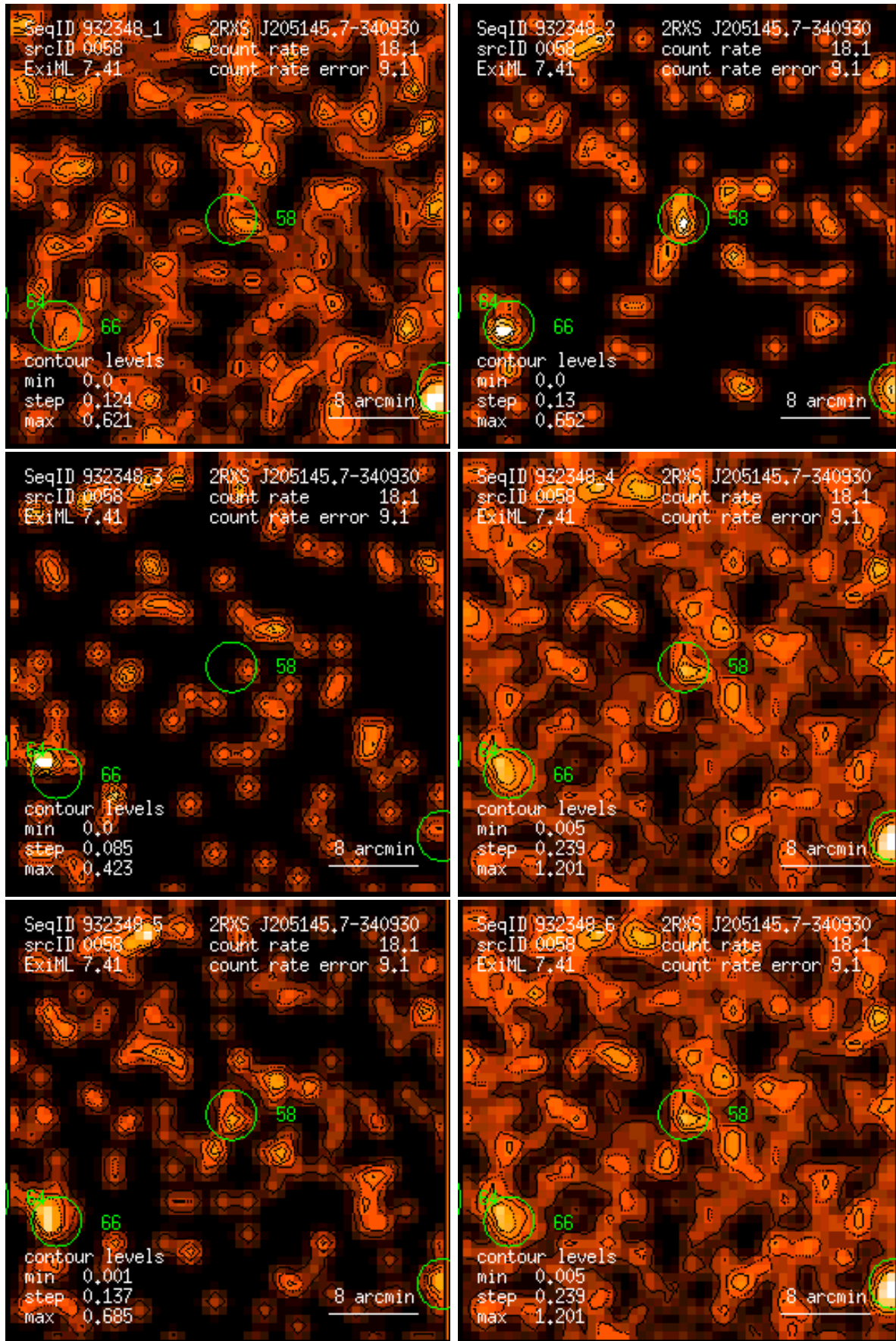
Figure 58: RASS 932348: detection 0058: band rate images, Gaussian filter: (1) PSPC channels 11 – 41, (2) 52 – 90, (3) 91 – 201, (4) 11 – 235, (5) 52 – 201, (6) 11 – 201. Broad band rates in counts/ks. Band rate contour levels in counts/ks/arcmin 2 .
