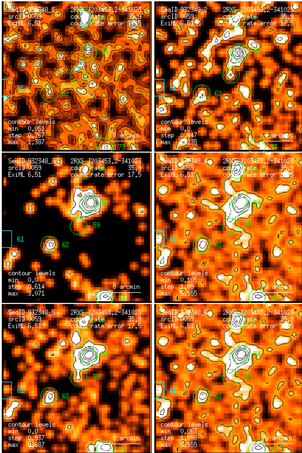
Figure 59: RASS 932348: detection 0059: band rate images, Gaussian filter: (1) PSPC channels 11 – 41, (2) 52 – 90, (3) 91 – 201, (4) 11 – 235, (5) 52 – 201, (6) 11 – 201. Broad band rates in counts/ks. Band rate contour levels in counts/ks/arcmin 2 .
