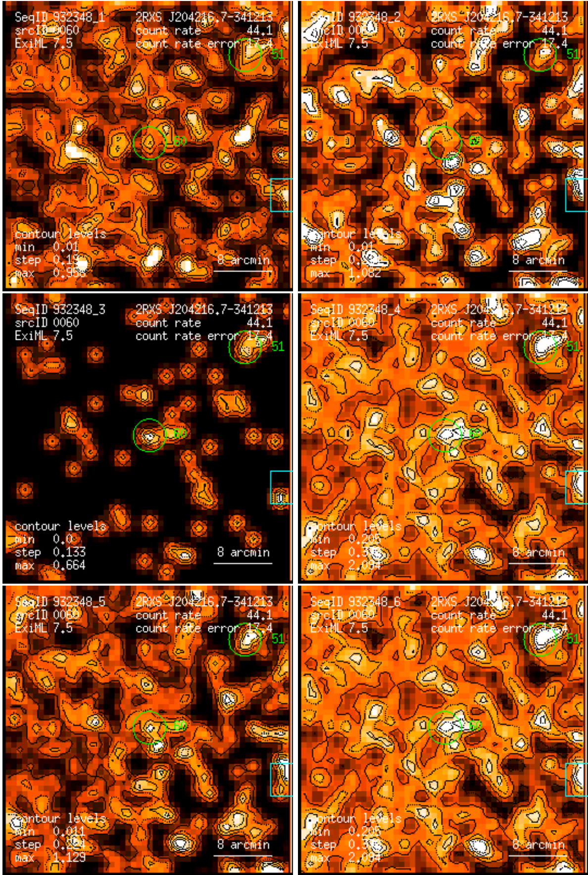
Figure 60: RASS 932348: detection 0060: band rate images, Gaussian filter: (1) PSPC channels 11 – 41, (2) 52 – 90, (3) 91 – 201, (4) 11 – 235, (5) 52 – 201, (6) 11 – 201. Broad band rates in counts/ks. Band rate contour levels in counts/ks/arcmin 2 .
