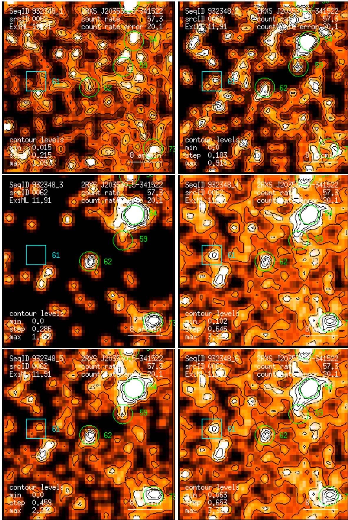
Figure 62: RASS 932348: detection 0062: band rate images, Gaussian filter: (1) PSPC channels 11 – 41, (2) 52 – 90, (3) 91 – 201, (4) 11 – 235, (5) 52 – 201, (6) 11 – 201. Broad band rates in counts/ks. Band rate contour levels in counts/ks/arcmin 2 .
