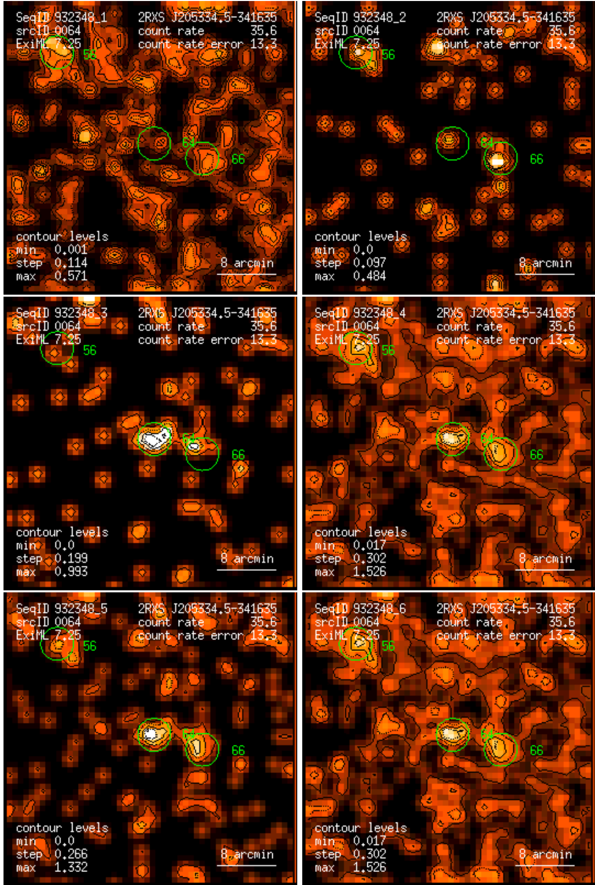
Figure 64: RASS 932348: detection 0064: band rate images, Gaussian filter: (1) PSPC channels 11 – 41, (2) 52 – 90, (3) 91 – 201, (4) 11 – 235, (5) 52 – 201, (6) 11 – 201. Broad band rates in counts/ks. Band rate contour levels in counts/ks/arcmin 2 .
