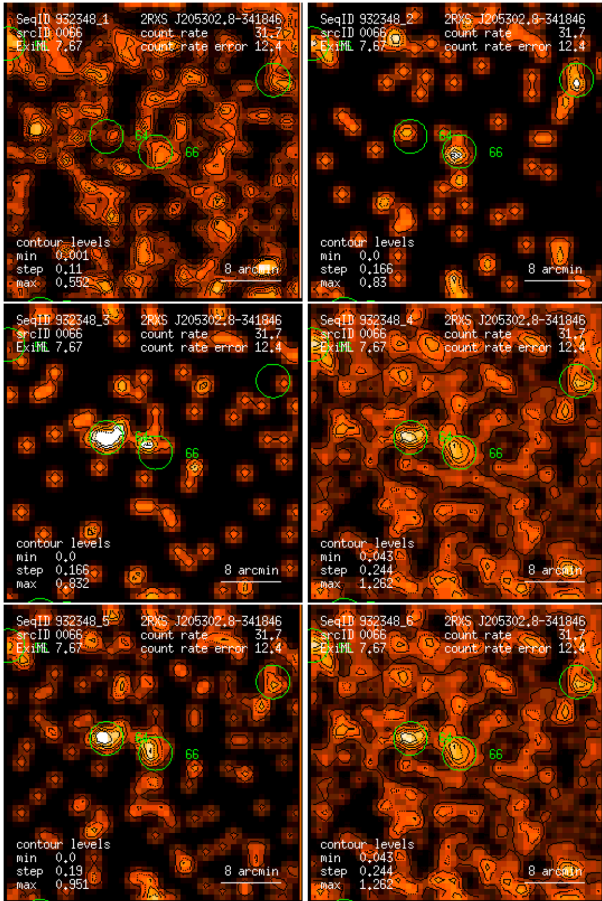
Figure 66: RASS 932348: detection 0066: band rate images, Gaussian filter: (1) PSPC channels 11 – 41, (2) 52 – 90, (3) 91 – 201, (4) 11 – 235, (5) 52 – 201, (6) 11 – 201. Broad band rates in counts/ks. Band rate contour levels in counts/ks/arcmin 2 .
